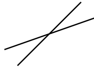
Figure 1. R(u) .
