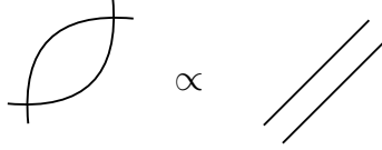
Figure 3. Unitarity.
