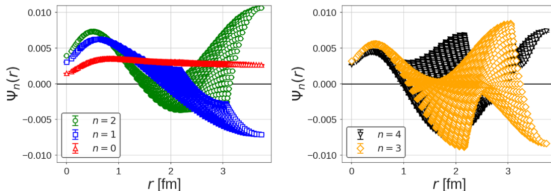
Figure 6. Eigenfunctions of elastic states in the A_1^+ representation of the HAL QCD Hamiltonian H^{LO} below the inelastic threshold \Psi_n(\vec{r}) on L = 48 at t/a = 13 for n = 0, 1, 2 (left) and n = 3, 4 (right), where red up-pointing triangles, blue squares, green circles, orange diamonds and black down-pointing triangles correspond to n = 0, 1, 2, 3 and 4 , respectively. The eigenfunction is normalized as \sum_{\vec{r}} |\Psi_n(\vec{r})|^2 = 1 and \Psi_n(\vec{0}) > 0 . Errors are statistical only.
