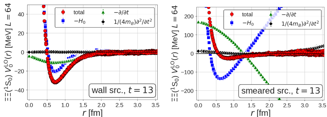
Figure 3. The potential at the leading order (LO) analysis V_0^{LO}(r) (red circles) from the wall source (left) and the smeared source (right) for \Xi\Xi(^1S_0) at t/a = 13 for L = 64 [20]. The blue squares, green triangles and black diamonds denote 1st, 2nd and 3rd terms in eq. (2.11), respectively.
