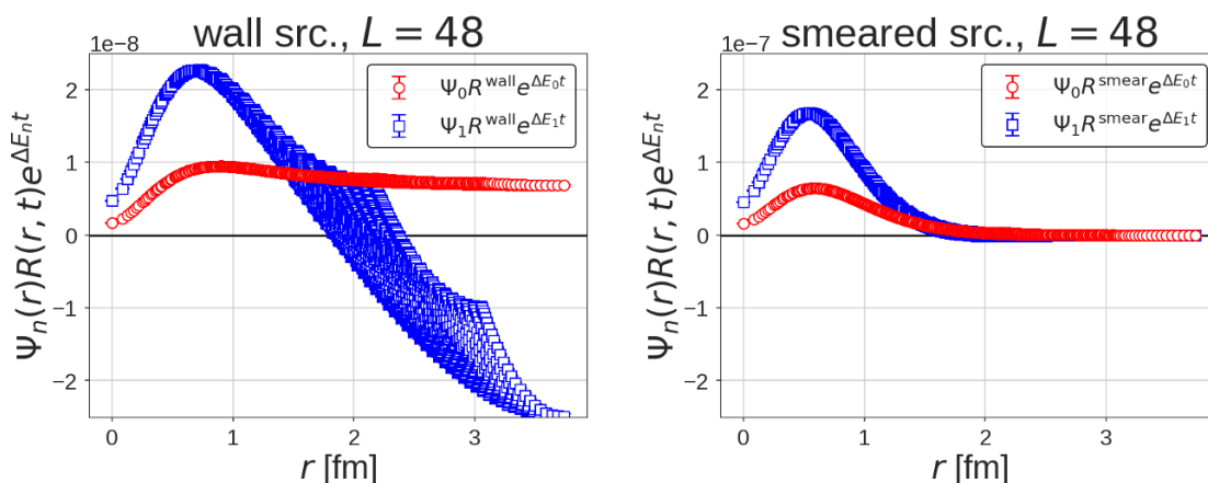
Figure 8. The overlap between the R -correlator and the eigenfunction, \Psi_n^\dagger(\vec{r})R(\vec{r}, t)e^{\Delta E_n t} , as a function of r at t/a = 13 on L = 48 for the ground state ( n = 0 , red circles) and the first excited state ( n = 1 , blue squares) in the case of the wall source (left) and the smeared source (right).
