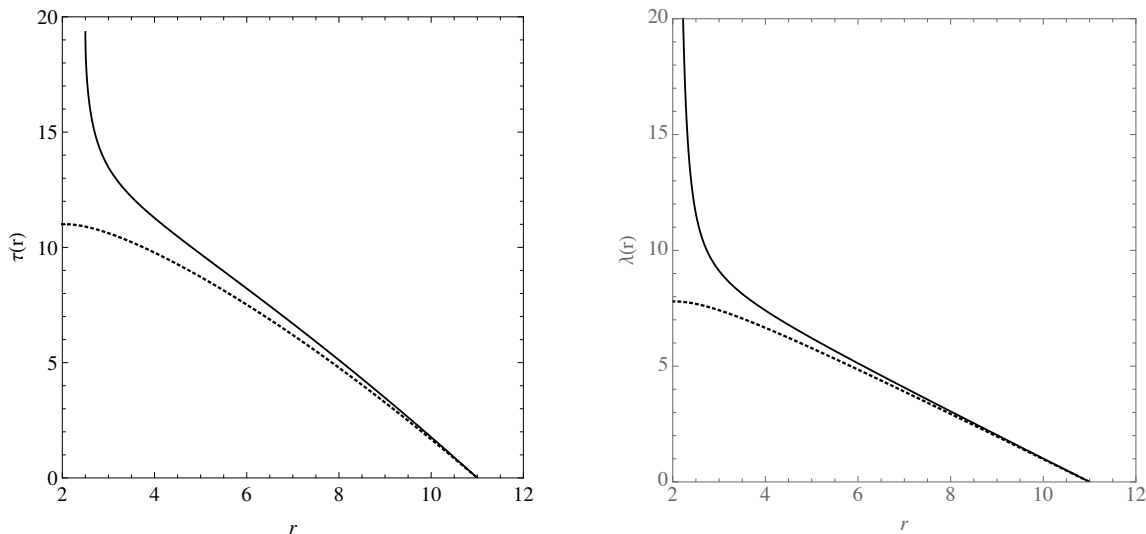
Figure 2. As in figure 1 for the \gamma -metric. The left panel shows the case for a massive particle, the right panel that for a massless one. In these plots, we assume E = M = L = n = 1 , \gamma = 2 , and r_{\text{in}} = 11 .
