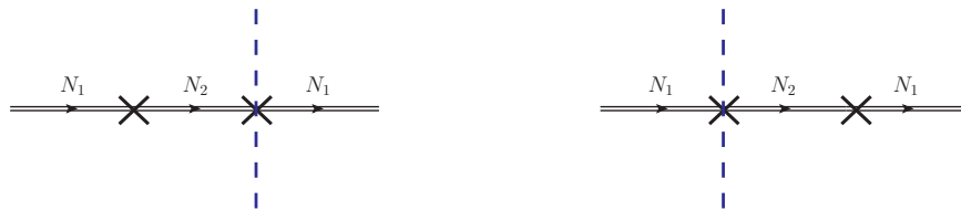
Figure 7. Diagrams showing in the EFT a neutrino of type 1 decaying into a lepton after mixing with a neutrino of type 2. The cross stands for the mixing vertex -\Gamma_{IJ}^{T=0}/2 . The cross with a cut selects the leptonic (or anti-leptonic) decay components: M(F_I^*F_J)/(16\pi) (or M(F_J^*F_I)/(16\pi) ). Propagators on the right of the cut are complex conjugate. Because the mixing vertex is real, circled and uncircled vertices coincide [30].
