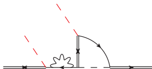
Figure 18. Diagram as in figure 15.
