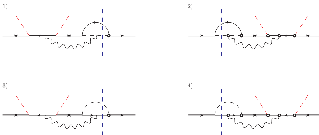
Figure 23. On each row we show the diagrams a) and b) of figure 19 together with their complex conjugates. Higgs bosons and leptons are cut.
