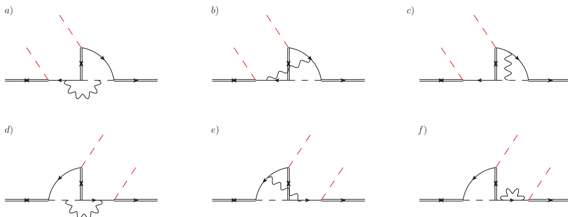
Figure 15. If the incoming and outgoing Majorana neutrinos are conventionally chosen to be of type 1, then the displayed diagrams contribute to a_{11}^{\ell} at order F^4 and at first order in the gauge couplings. The diagrams contribute also to a_{11}^{\ell} if cut through the anti-lepton. Only diagrams proportional to (F_1^* F_2)^2 are displayed.
