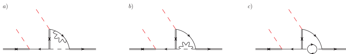
Figure 16. Diagrams as in figure 15. In diagram c ), the particles in the small loop coupled to a Higgs boson are a top-quark and a heavy-quark doublet.
