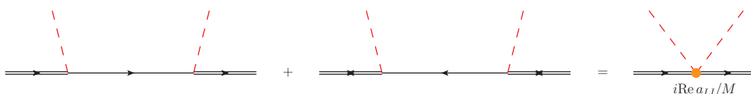
Figure 6. On the left-hand side the diagrams in the fundamental theory that match the real part of a_{IJ} at order F^2 (right-hand side). Red dashed lines indicate external Higgs bosons with a soft momentum much smaller than the mass of the Majorana neutrinos.
