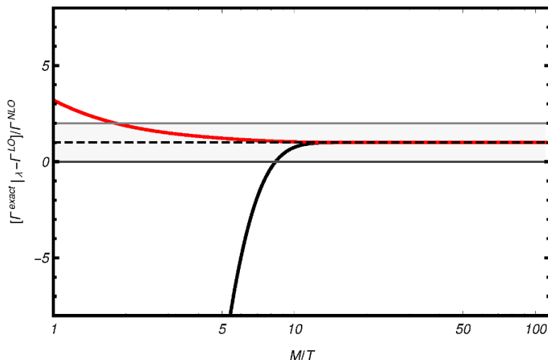
Figure 29. The black line shows the difference between the exact neutrino production rate up to order \lambda (top-Yukawa and gauge couplings set to zero) and the neutrino production rate at leading order in T/M divided by the neutrino production rate at next-to-leading order in T/M . The red line is as above but with the leading-order neutrino production rate multiplied by (1 + n_B(M/2) - n_F(M/2)) . The neutrino is taken at rest. The one-loop running four-Higgs coupling, \lambda , is taken \lambda(10^7 \text{ GeV}) \approx 0.02 ( \lambda(125 \text{ GeV}) \approx 0.126 ) [45].
