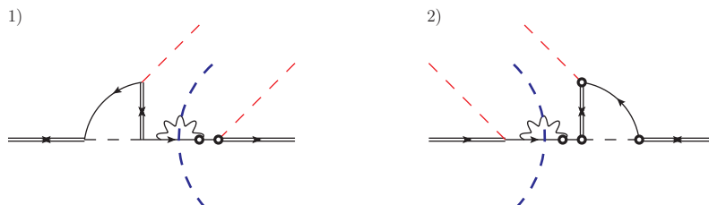
Figure 22. Diagram f ) of figure 15 together with its complex conjugate. Gauge bosons and leptons are cut.
