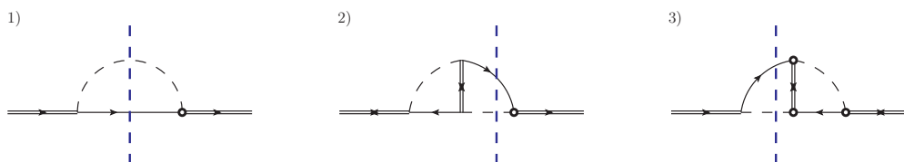
Figure 3. One-loop and two-loops self-energy diagrams in the fundamental theory (2.1) contributing to the decay of a heavy Majorana neutrino into leptons. Vertical blue dashed lines are the cuts selecting a final state made of a Higgs boson and a lepton. Circled vertices and propagators are defined in appendix B.1.
