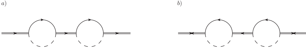
Figure 9. Two-loop self-energy diagrams in the fundamental theory contributing to the indirect CP asymmetry at T = 0 in the flavoured case only. Diagram a) admits two cuts through lepton lines, whereas diagram b) admits two cuts through anti-lepton lines.
