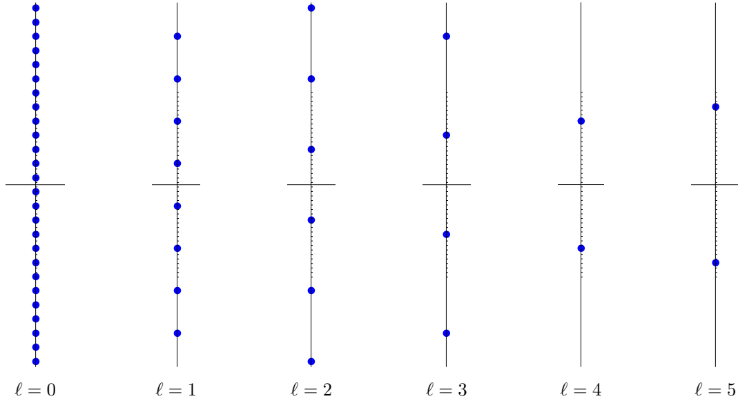
Figure 2. Singularities in the complex Borel plane for ABJM gauge theory on S^3 (at large level k , and with rank of the gauge group N = 2 ). Every vertical line in this figure should be seen as the very same imaginary axis, i.e., all singularities are along the same line (they are shown separately just to make manifest the existence of different “instanton” actions A_\ell , for \ell = 1, 2, 3, 4, 5 ).
