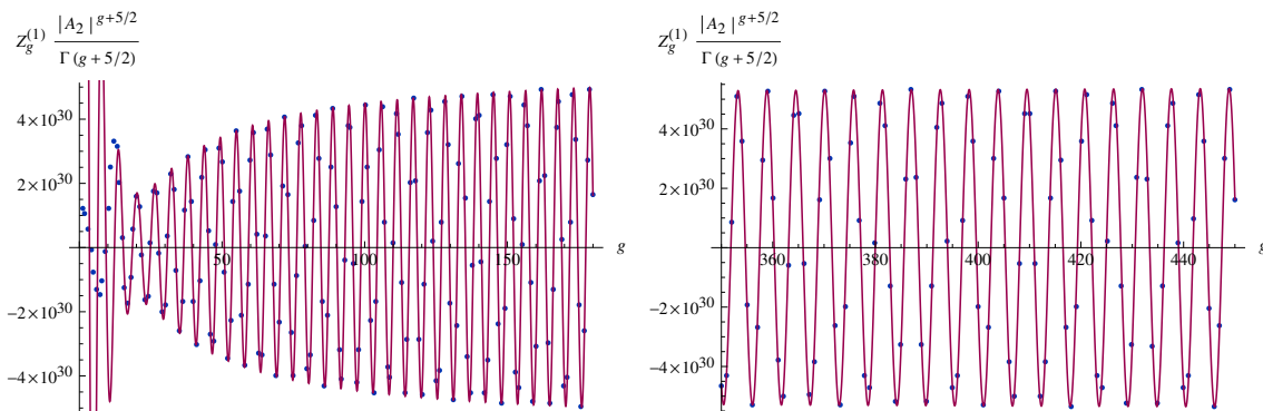
Figure 8. Numerical analysis of the exponentially subleading large-order behavior of the coefficients Z_g^{(0)} , for a value of the mass parameter M = 3.2 and A_2 = \frac{1}{2}A(4 + M^2) , corresponding to the leading behavior of the redefined coefficients Z_g^{\{1\}} . Left and right plots show both the numerical value of these coefficients (the dots) as well as their analytically predicted large-order behavior (the solid line), for small and large g , respectively. The agreement is clearly excellent at large order.
