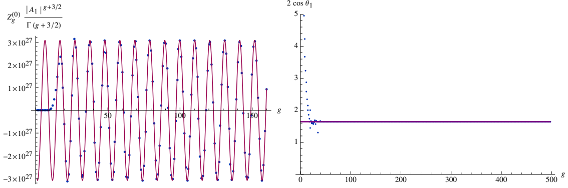
Figure 7. Numerical analysis of the leading large-order behavior of the coefficients Z_g^{(0)} , for values of the mass parameter M = 3.2 , and A_1 = \frac{1}{2}A(1 + M^2) . On the left, both the numerical value of these coefficients (the dots) and their predicted analytical behavior (the solid line) are shown. On the right, we plot the convergence towards 2 \cos \theta_{1,+} of a particular combination of the coefficients, the one given in (3.68), where \theta_{1,+} is the angle associated with the first instanton action s_1 . The agreement is excellent.
