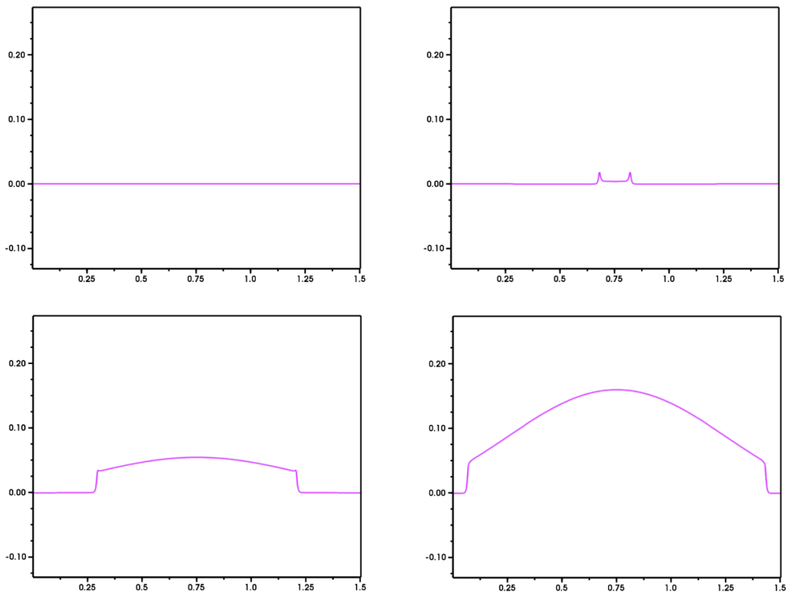
Figure 6. The deviation from free passage for the snapshots in figure 5, computed as the difference between the actual field solution and free passage solution.
