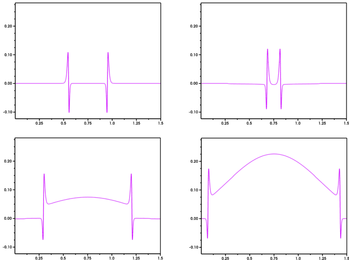
Figure 4. For each snap shot in figure 3 we plot the corresponding deviation from free passage, merely computed as the difference between the actual field solution and the free passage solution. Notice that the shape of the instability is similar to the ground state of a finite square well thus supporting our heuristic argument in section 3. The kinks at the wall locations indicate that the soliton approximation, (4.4), produces a slightly wider soliton than the true one. The persistence of the kinks throughout the snapshots means that the approximate walls stay intact. Thus, retreat to the original bubble vacuum does not result from collapse of the walls, but rather from evolution of the field inside the collision region. The former behavior would not be an example of our effect since the ground state is nearly zero at the walls. Instead, it would be the “temporary excursion” observed by [3, 4] at insufficiently relativistic speeds.
