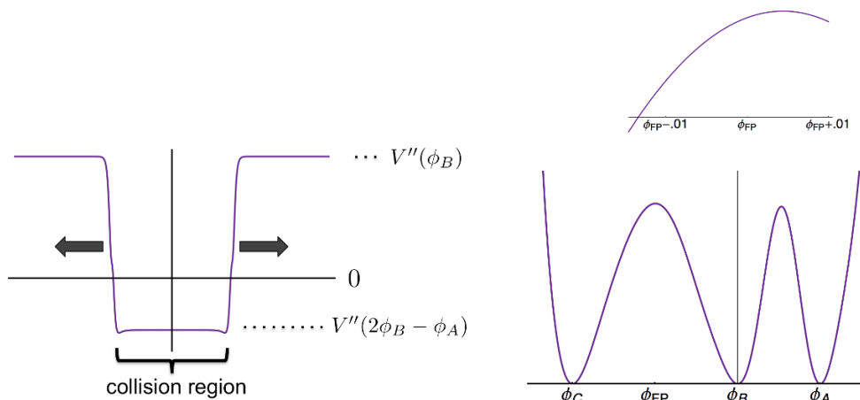
Figure 1. To the left is an example of an analog quantum potential after collision. This analog potential is typical of models that permit unstable mode(s). The particular collision this is associated with is pictured in figures 3 and 4. The model’s potential for this collision is shown on the right, with a magnified plot near the free passage field value also included in the upper right corner.
