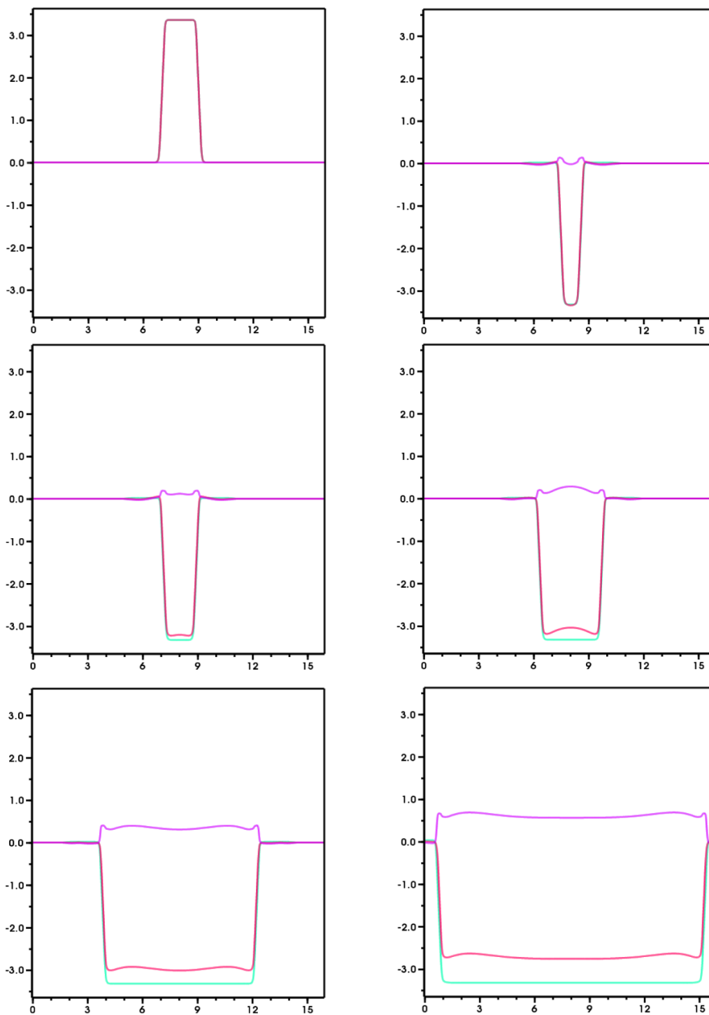
Figure 8. Above are snap shots of the collision of two \phi_B bubbles nucleated in parent \phi_A for the potential pictured in figure 7. The field is plotted in red, the free passage solution in green, and the deviation in purple. The field in the collision region is kicked via free passage to a location where -V' is negative, yet nonetheless retreats in the positive direction — running through an entire interval where -V' is negative — ultimately back to the original bubble’s basin of attraction.
