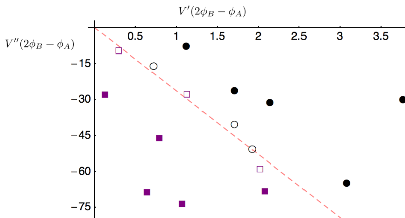
Figure 2. The results of numerical simulations for various values of V'(2\phi_B - \phi_A) and V''(2\phi_B - \phi_A) . Cases where the field retreats back toward \phi_B are indicated by a purple square while those that continue toward \phi_C are indicated by black circles. Note that there is a rough boundary that separates the two classes. We’ve unshaded the simulations deemed to lie along this boundary, and plotted a least squares fit to these points which has slope -26.5 .
