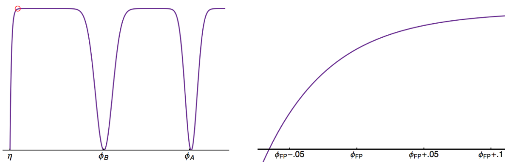
Figure 7. To the left is a plot of the potential given by (5.2) with parameter values \eta = -3.5 , K = 20 , k_1 = 10 , k_2 = 5 , \phi_A = 3.25 and \phi_B = 0 . On the right we include a magnified plot of the potential near the free passage field location, 2\phi_B - \phi_A (circled in red on the unmagnified plot). The results of a soliton–anti-soliton collision for this model are pictured in figure 8.
