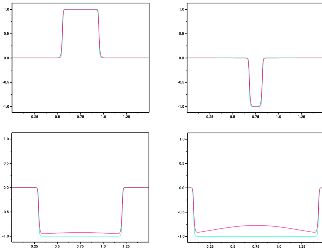
Figure 3. Shown above are snapshots taken during a collision that is representative of those where the field retreats back to \phi_B despite temporarily migrating into basin of attraction of the minimum at -2 after the collision. The solution to the field’s EOM, in red, is plotted over the free passage solution, in green. (Note: solitons in the field’s initial conditions were approximated by (4.4), whereas those used in the free passage solution were constructed by numerical inversion as discussed in the footnote on page 9. As noted, the effect of using the more exact numerical approach is minimal.)
