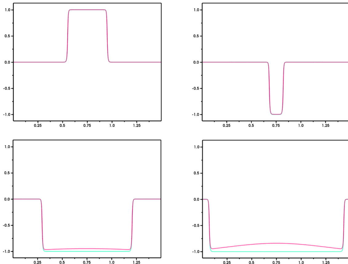
Figure 5. Results of the same collision pictured in figure 3, only with solitons in the field’s initial conditions constructed using the more accurate method described in the footnote on 9. All parameter values, including initial wall locations, and speed, were identical for the two runs. The solution to the field’s EOM is in red, and the free passage solution is in green.
