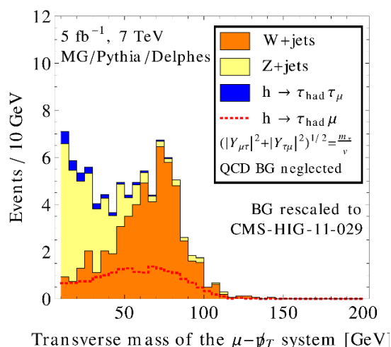
Figure 11. The transverse mass distribution of the muon-missing energy system for the backgrounds and for the \tau_{\text{had}}\mu signal.
