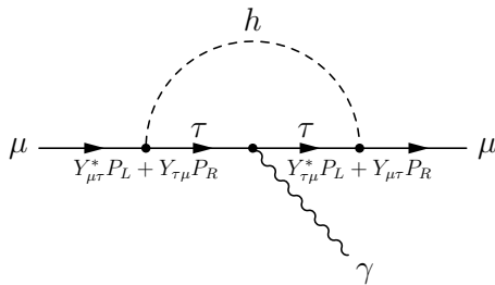
Figure 4. A diagram contributing to the anomalous magnetic moment g - 2 of the muon through FV couplings of the Higgs to \tau\mu .
