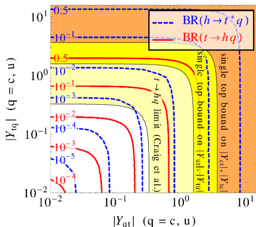
Figure 8. Predictions for various flavor changing neutral current (FCNC) processes mediated by the flavor violating Yukawa couplings Y_{ct} , Y_{tc} or Y_{ut} , Y_{tu} of a 125 GeV Higgs boson. Where appropriate, we have approximated the diagonal Yukawa couplings by their Standard Models values. Blue dashed contours indicate the branching ratio for h \rightarrow t^*q , red solid contours the one for t \rightarrow hq (where q denotes a charm or up quark). The light yellow region shows a recent limit on t \rightarrow hc (or hu ) from an LHC multi-lepton search [50].
