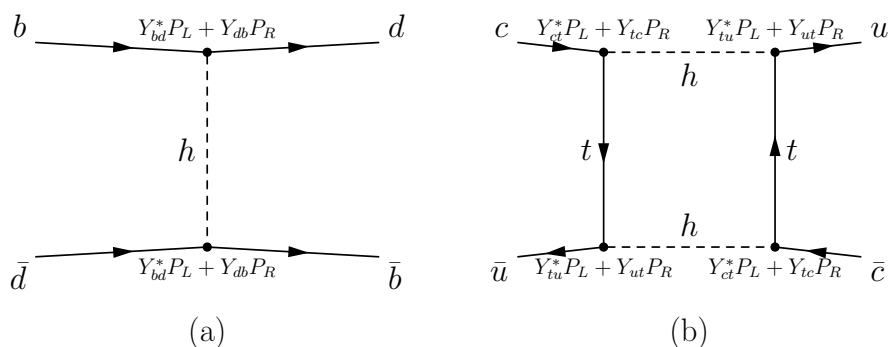
Figure 7. Two representative diagrams through which flavor violating Higgs Yukawa couplings can contribute to neutral meson mixing.
