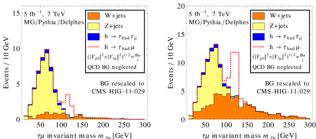
Figure 10. Signal and background rates for h \rightarrow \tau\mu events in a CMS-like search (see text) as a function of the reconstructed \mu - \tau invariant mass m_{\tau\mu} for a vector boson fusion-enriched event sample. In the left panel the transverse mass cut m_T(\mu, \mathbf{p}_{\text{miss},T}) < 40 GeV is included, while in the right panel it is omitted. The QCD multijet background and the small t\bar{t} background, are not included. The value chosen for \sqrt{Y_{\tau\mu}^2 + Y_{\mu\tau}^2} is well within the region allowed by other searches for flavor violation in the \mu - \tau system (see section 3).
