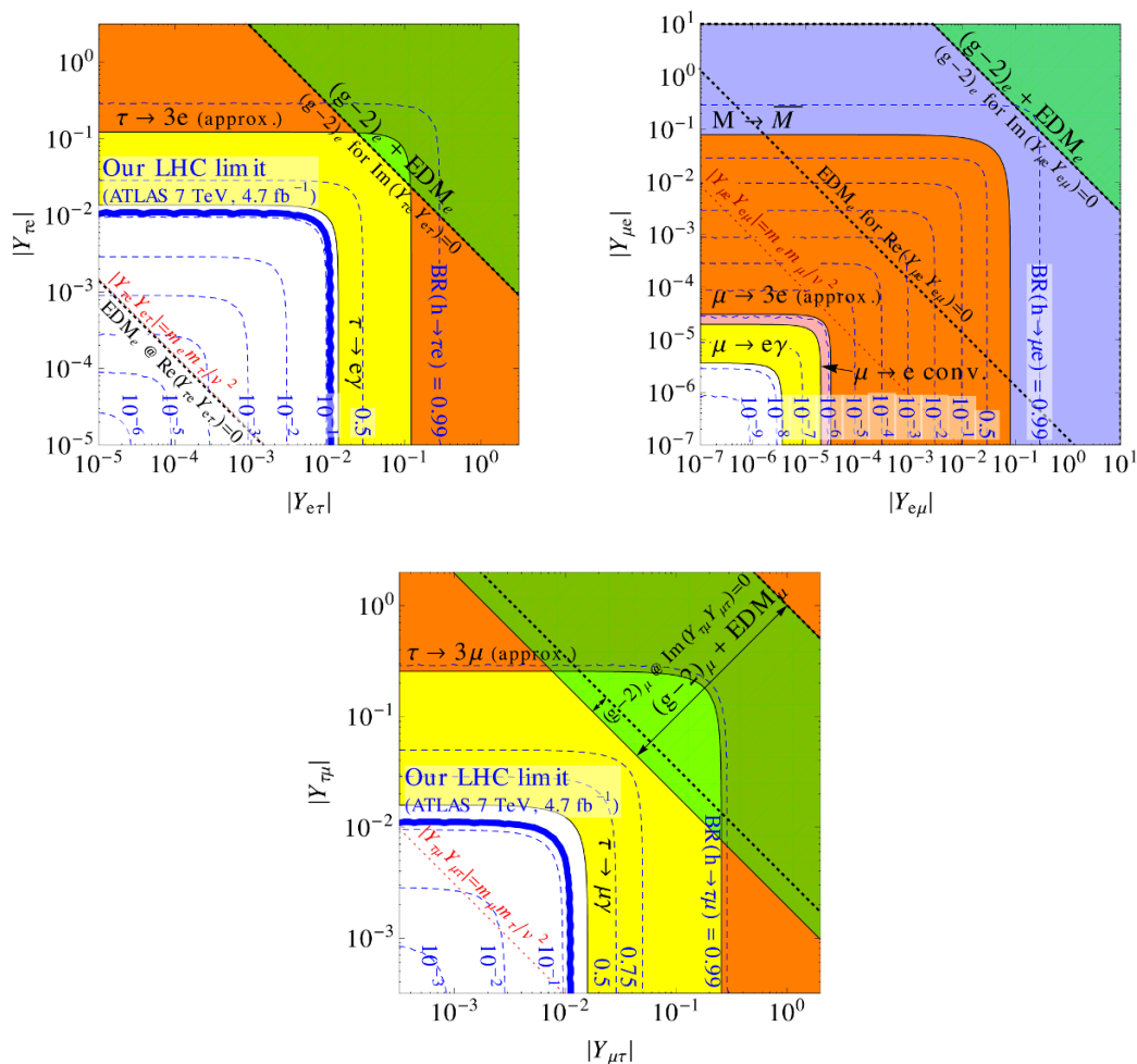
Figure 6. Constraints on the flavor violating Yukawa couplings |Y_{e\tau}| , |Y_{\tau e}| (upper left panel), |Y_{e\mu}| , |Y_{\mu e}| (upper right panel) and |Y_{\mu\tau}| , |Y_{\tau\mu}| (lower panel) of a 125 GeV Higgs boson. The diagonal Yukawa couplings are approximated by their SM values. Thin blue dashed lines are contours of constant BR for h \rightarrow \tau e , h \rightarrow \mu e and h \rightarrow \tau \mu , respectively, whereas thick blue lines are the LHC limits derived in section 5.1. (These limits could be greatly improved with dedicated searches on existing LHC data, see section 5.3.) Shaded regions show the constraints discussed in section 3 as indicated in the plots. Note that g - 2 [EDM] searches (diagonal black dotted lines) are only sensitive to parameter combinations of the form \text{Re}(Y_{\alpha\beta}Y_{\beta\alpha}) [ \text{Im}(Y_{\alpha\beta}Y_{\beta\alpha}) ]. We also show limits from a combination of g - 2 and EDM searches with marginalization over the complex phases of the Yukawa couplings (green shaded regions). Note that (g - 2)_\mu provides upper and lower limits (as indicated by the double-sided arrows in the lower panel) if the discrepancy between the measurement and the SM prediction [38, 43] is taken into account. The thin red dotted lines show rough naturalness limits Y_{ij}Y_{ji} \lesssim m_i m_j / v^2 (see section 2).
