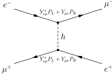
Figure 3. Diagram leading to muonium-antimuonium oscillations.
