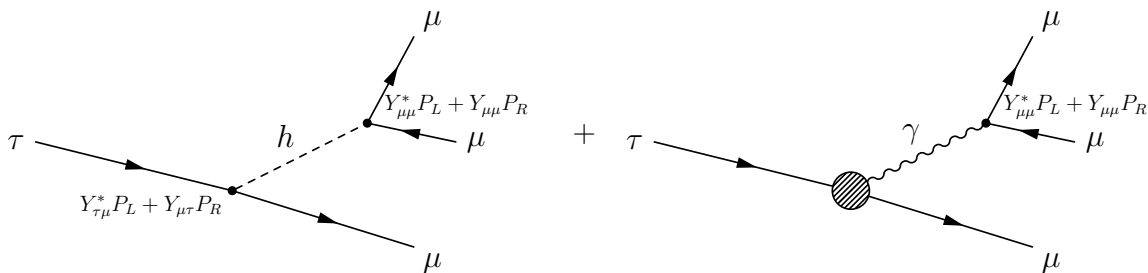
Figure 2. Diagrams leading to \tau \rightarrow 3\mu decay. The tree level Higgs exchange contribution (left) is typically subdominant compared to higher-order contributions with the topology shown on the right. The blob represents loops of the form shown in figures 1 and 12.
