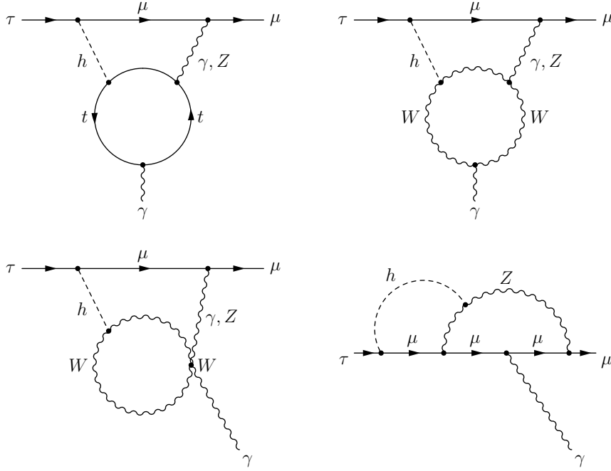
Figure 12. 2-loop diagrams contributing to \tau \rightarrow \mu\gamma .
