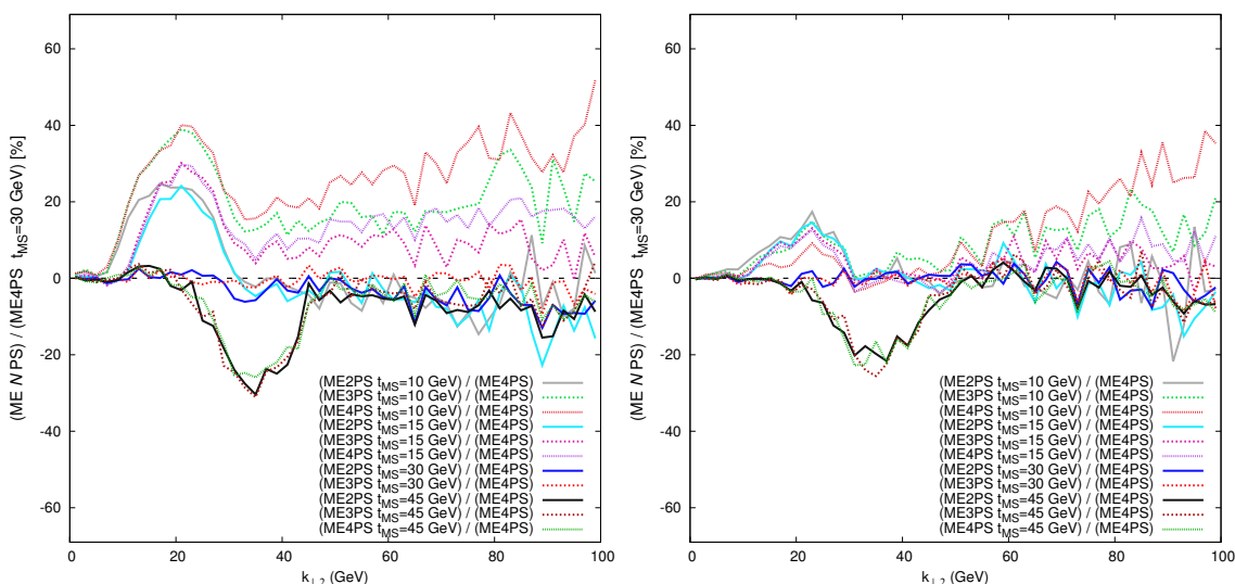
Figure 14. k_{\perp,2} separation of the second jet in W +jets events at E_{\text{CM}} = 1960 GeV in p\bar{p} collisions. The curves are normalised to the k_{\perp,2} distribution in ME4PS at t_{\text{MS}} = 30 GeV. Jets were defined with the k_{\perp} -algorithm with D = 0.4 . Multiple interactions and hadronisation were switched off. Left panel: plots produced with PYTHIA8 Tune 4C. Right panel: plots produced with PYTHIA8 Tune 4C, with enforced rapidity ordering switched off.
