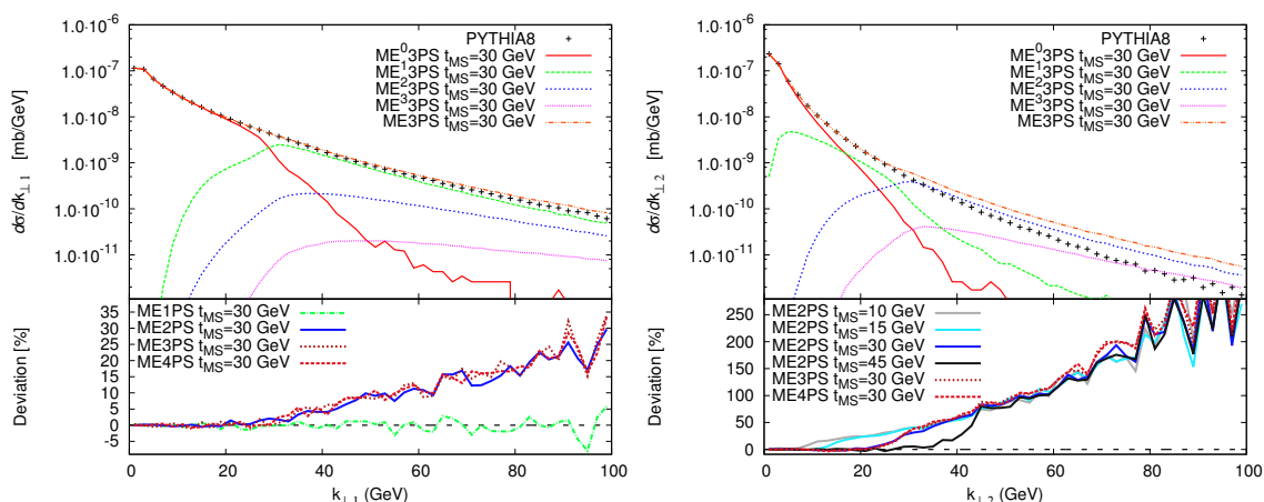
Figure 13. k_{\perp} of the hardest and second hardest jet, for different number of merged jets, in W +jets events at E_{\text{CM}} = 1960 \text{ GeV} in p\bar{p} collisions. The merging scale is defined in t_{\text{MS}} = \min\{k_{\perp i}\} . Jets were defined with the k_{\perp} -algorithm with D = 0.4 . Multiple interactions and hadronisation were switched off. Plots produced with PYTHIA8 Tune 4C. The bottom in-sets show the deviation of the merged samples from default, first-order corrected PYTHIA8.
