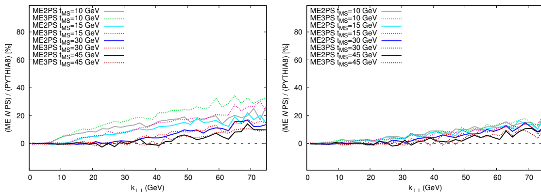
Figure 9. Comparison of the k_{\perp} of the first jet in W +jets events at E_{\text{CM}} = 1960 GeV in p\bar{p} collisions, between default, first-order corrected PYTHIA8, and CKKW-L, for different number of merged jets and different merging scales. Jets were defined with the k_{\perp} -algorithm with D = 0.4 , clustering to exactly one jet. Multiple interactions and hadronisation were switched off. Left panel: results when using Tune 4C, which by default includes ordering emissions in rapidity as well as \rho . Right panel: results when using Tune 4C, with enforced rapidity ordering switched off.
