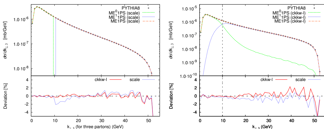
Figure 5. A comparison of different prescriptions of choosing the history for e^+e^- \rightarrow 3 jets. Results for choosing in a probabilistic way, with splitting probabilities defined in eqs. (B.10) and (B.11), are labelled “ckkw-l”, while adopting a winner-takes-it-all strategy of picking the history with lowest scale carries the label “scale”. The plots were produced with a merging scale t_{\text{MS}} = \min\{k_{\perp i}\} = 10 GeV. Hadronisation was switched off. The left panel shows the k_{\perp} -separation (in the Durham algorithm) between the third and second hardest parton in the first (reconstructed) emission. The distributions for ME 0 1PS and ME 1 1PS for a scale-dependent choice are shown in the upper part, whereas the bottom in-set gives the deviation of both prescriptions from default PYTHIA8. In the right panel we show the k_{\perp} -separation the third and second hardest jets defined in the exclusive Durham algorithm for the probabilistic approach, with the bottom in-set again giving the deviation of both prescriptions from default PYTHIA8.
