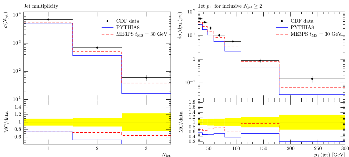
Figure 12. Jet multiplicity and inclusive jet transverse momentum in Drell-Yan events, as measured by CDF [26]. The merging scale is t_{\text{MS}} = 30 \text{ GeV} . Effects of multiple scatterings and hadronisation are included, and Tune 4C was chosen. The plots were produced with RIVET [24].
