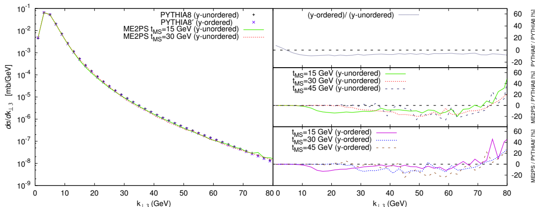
Figure 20. k_{\perp,3} separation of the third jet in pure QCD jet events at E_{CM} = 1960 GeV in p\bar{p} collisions, for three different merging scales. Jets were defined with the k_{\perp} -algorithm with D = 0.4 . Multiple interactions and hadronisation were switched off. Curves with enforced rapidity ordering in the shower carry the label “y-ordered”, while results without explicit rapidity ordering are labelled “y-unordered”. Left panel: k_{\perp,3} separation of the third jet. Upper right panel: deviation in k_{\perp,3} between default PYTHIA8 (Tune 4C) and PYTHIA8 (Tune 4C) with no enforced rapidity ordering. Centre right panel: deviation in k_{\perp,3} between ME2PS sample and PYTHIA8 (Tune 4C) with no enforced rapidity ordering. Lower right panel: deviation in k_{\perp,3} between ME2PS sample and default PYTHIA8 (Tune 4C).
