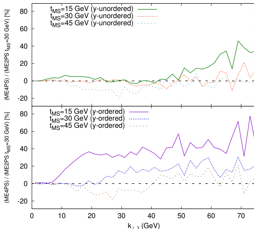
Figure 19. k_{\perp 3} separation of the second and third jet in W +jets events at E_{CM} = 1960 GeV in p\bar{p} collisions. The curve shows the deviation in k_{\perp 3} of ME4PS for three different merging scales, with respect to ME2PS for t_{MS} = 30 GeV. Jets were defined with the k_{\perp} -algorithm with D = 0.4 . Hadronisation and multiple interactions were switched off. Curves with enforced rapidity ordering in the shower carry the label “y-ordered”, while results without explicit rapidity ordering are labelled “y-unordered”.
