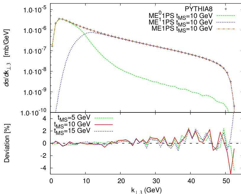
Figure 3. k_{\perp} separation of the third jet in e^+e^- collisions at E_{CM} = 91.25 GeV. Jets were defined with the Durham algorithm. Hadronisation was switched off. The bottom in-set shows the deviation of the merged samples for three different merging scales t_{MS} with respect to default, matrix-element-corrected PYTHIA8.
