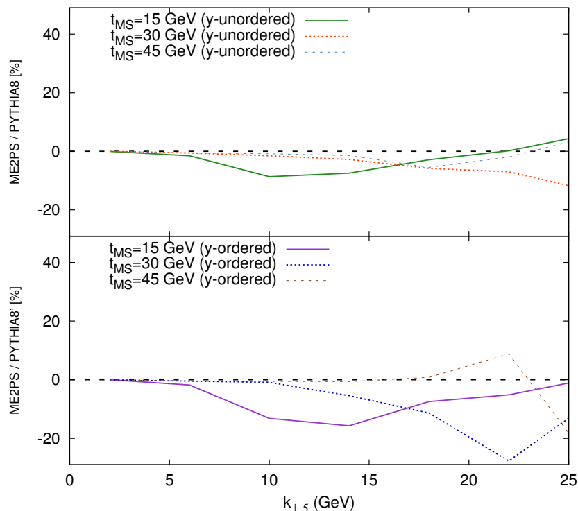
Figure 21. k_{\perp 5} separation between the fourth and fifth jet in di-jet events at E_{CM} = 1960 GeV in p\bar{p} collisions. The curves show the deviation of k_{\perp 5} -distributions in ME2PS for three different merging scales, with respect to PYTHIA8. Jets were defined with the k_{\perp} -algorithm with D = 0.4 . Hadronisation and multiple interactions were switched off. Curves with enforced rapidity ordering in the shower carry the label “y-ordered”, while results without explicit rapidity ordering are labelled “y-unordered”.
