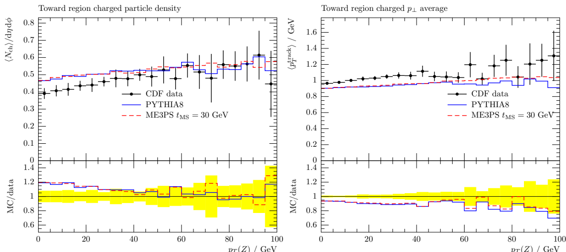
Figure 16. Toward region charged particle density and average p_{\perp} in Drell-Yan events, as measured by CDF [27]. The merging scale is t_{MS} = \min\{k_{\perp i}\} = 30 GeV. Effects of multiple scatterings and hadronisation are included, and Tune 4C was chosen. The plots were produced with RIVET [24].
