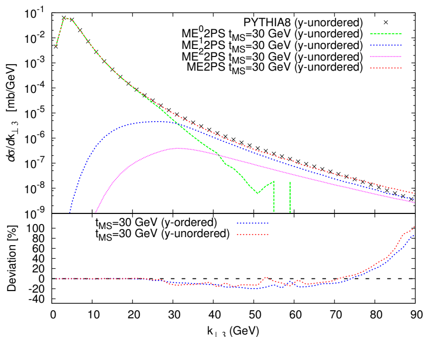
Figure 18. k_{\perp 3} separation of the third jet in pure QCD jet events at E_{CM} = 1960 GeV in p\bar{p} collisions. The merging scale is t_{MS} = 30 GeV. Jets were defined with the k_{\perp} -algorithm with D = 0.4 . Multiple interactions are included and hadronisation was switched off. Curves with enforced rapidity ordering in the shower carry the label “y-ordered”, while results without explicit rapidity ordering are labelled “y-unordered”. The bottom in-set shows the deviation of the merged sample default PYTHIA8.
