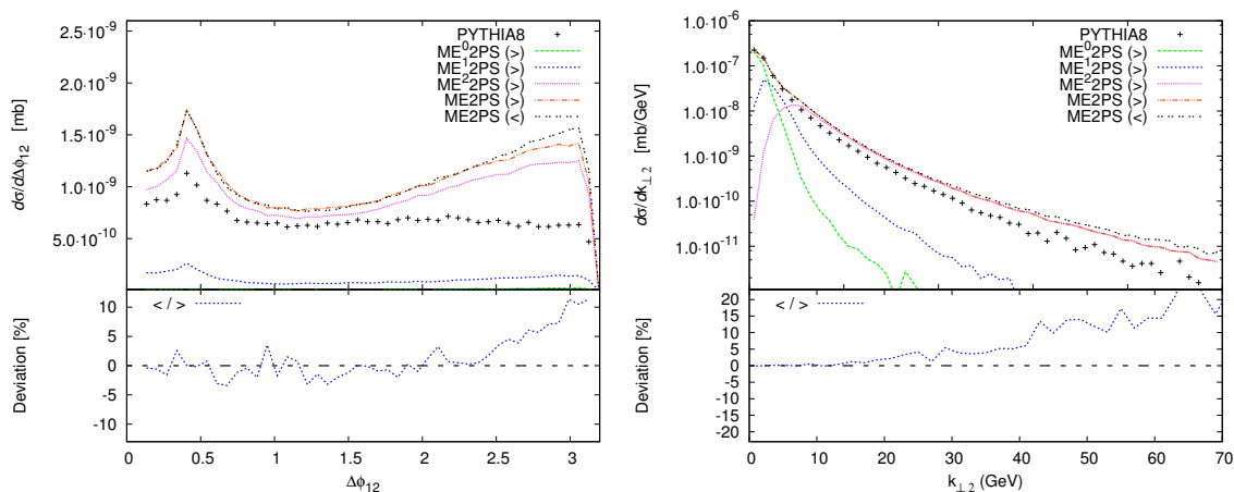
Figure 6. Two different ways of choosing a combined scale for unordered emissions, in W + 2 jet events at E_{\text{CM}} = 1960 GeV in p\bar{p} collisions. The merging scale is t_{\text{MS}} = 10 GeV. The curves are labelled with “>” when assigning the higher scale \rho_{\text{combined}} = \max(\rho_i, \rho_{i+1}) , and with “<” when assigning the lower scale \rho_{\text{combined}} = \min(\rho_i, \rho_{i+1}) , as the combined scale of two unordered emissions. The bottom in-sets show the deviation of the lower scale sample with respect to the higher scale sample. Jets were defined in the k_{\perp} -algorithm with D = 0.4 , while multiple scatterings and hadronisation were turned off. The left panel shows the azimuthal difference \Delta\phi_{12} between the hardest and second hardest jet. The right panel shows the k_{\perp} separation k_{\perp,2} of the second hardest jet.
