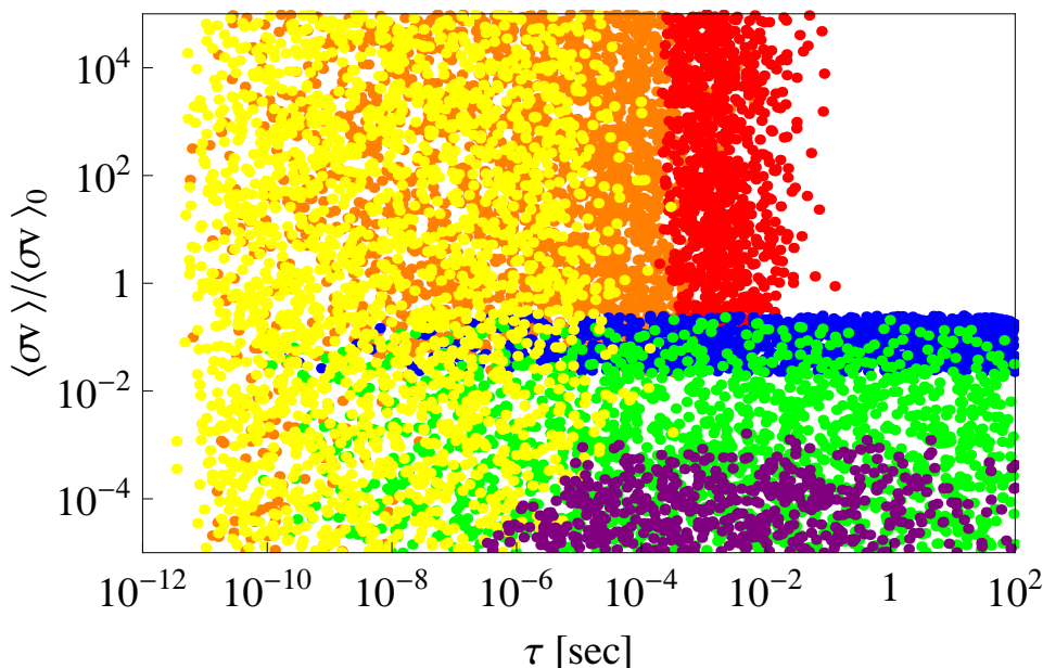
Figure 1. As shown in [3], hidden sector DM can arise through a handful of production mechanisms, each corresponding to a distinct window in the \tau - \langle\sigma v\rangle plane. Here {FO&D, FO&D r , FO&D a , FI, FI r , FI a } are denoted by {blue, green, purple, red, orange, yellow}. The re-annihilation mechanisms {FO&D r , FI r } occur when a sufficiently large abundance of X' particles are produced in FO&D or FI such that X' annihilation starts up again. Meanwhile, the mechanisms {FO&D a , FI a } result when the FO&D and FI processes generate a particle anti-particle asymmetry for X' . Every point corresponds to the observed DM abundance of \Omega h^2 = 0.11 and we have inclusively scanned over the remaining parameters relevant to the cosmological evolution, including 10 \text{ GeV} < m < 1 \text{ TeV} and 1/20 < m'/m < 1/2 . See [3] for details.
