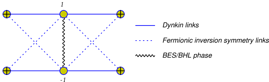
Figure 4. The Dynkin diagram for the quantum Bethe equations.
