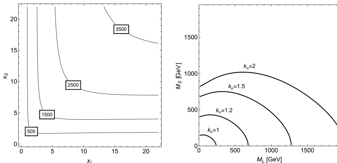
Figure 4. Left: contours of k_u^{-4}\delta m_h^2 in \text{GeV}^2 in the (x_L, x_S) plane, according to (4.1). Right: contours of \Delta = 20 in the (M_L, M_S) plane for different values of k_u that have a Higgs mass at 125 GeV.
