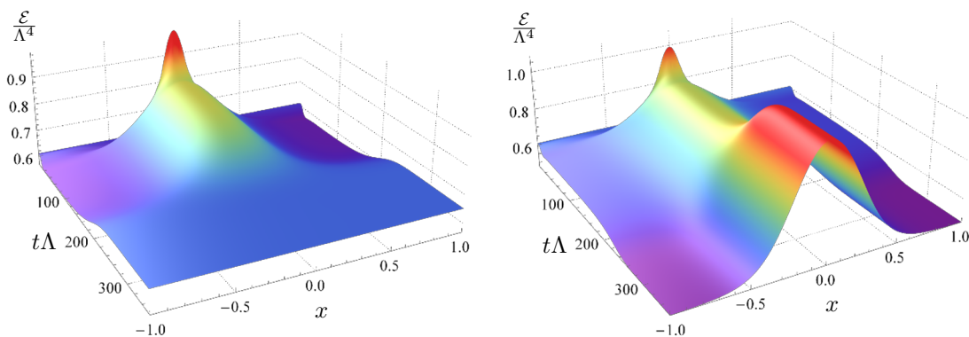
Figure 28. Extension to longer times of the time evolution shown in figure 24(bottom-left), whose initial state is a homogeneous configuration plus a large perturbation of amplitude \mathcal{A} . At intermediate times this generates the unstable solution \mathcal{X}_c plus a small perturbation. (Left) If the amplitude of the initial perturbation \mathcal{A} is slightly smaller than the critical value \mathcal{A}^* then the system eventually evolves back to the homogeneous solution labelled as \mathcal{X}_d in figure 27. (Right) If the amplitude of the initial perturbation \mathcal{A} is slightly larger than the critical value \mathcal{A}^* then the system eventually evolves towards the stable, inhomogeneous solution labelled as \mathcal{X}_e in figure 27.
