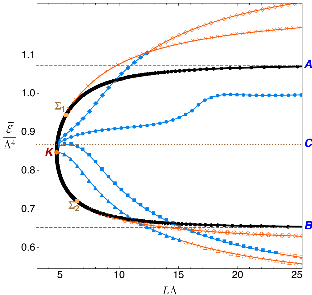
Figure 15. Same stability diagram as in figure 8 with the inclusion of some lumpy-brane curves that bifurcate from the GL merger curve. These curves have constant \hat{T} given by \{\hat{T}_\times, \hat{T}_\otimes, \hat{T}_\blacklozenge, \hat{T}_\bullet, \hat{T}_\blacksquare, \hat{T}_\blacktriangle\} \simeq \{0.390711, 0.405141, 0.395420, 0.395894, 0.396367, 0.397307\} . Solid blue markers (empty orange markers), no matter their shape, indicate positive (negative) \Delta\hat{\sigma}|_{\text{same}\hat{L},\hat{\rho}} .
