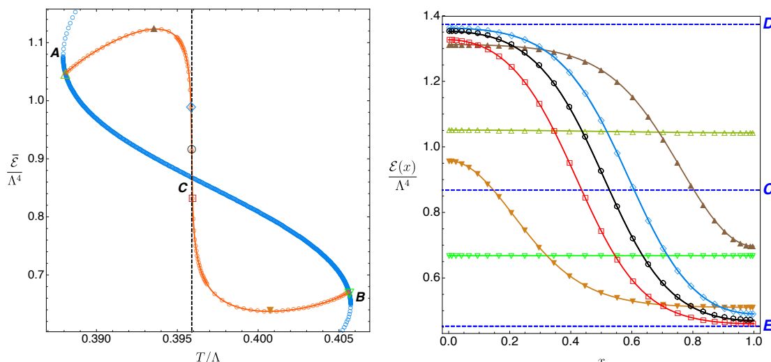
Figure 13. Lumpy branes at constant \hat{L} \simeq 11.501849 . (Left) \hat{\mathcal{E}} as a function of \hat{T} . This figure reproduces figure 11 but this time it singles out only the relevant lumpy brane with \hat{L} = \hat{L}_\circ \simeq 11.501849 (orange circles) and the uniform branes (blue circles) and zooms in on the relevant region. It also identifies 7 solutions whose energy density profiles are then plotted on the right panel. From left to right these are given by: (\hat{T}, \hat{\mathcal{E}})_\Delta \simeq (0.388085, 1.047078) , (\hat{T}, \hat{\mathcal{E}})_\blacktriangle \simeq (0.393560, 1.123216) , (\hat{T}, \hat{\mathcal{E}})_\diamond \simeq (0.395846, 0.988820) , (\hat{T}, \hat{\mathcal{E}})_\circ \simeq (0.3958945, 0.914833) , (\hat{T}, \hat{\mathcal{E}})_\square \simeq (0.395941, 0.831460) , (\hat{T}, \hat{\mathcal{E}})_\blacktriangledown \simeq (0.400765, 0.637410) , (\hat{T}, \hat{\mathcal{E}})_\nabla \simeq (0.405648, 0.667817) . (Right) Energy density profile \hat{\mathcal{E}}(x) for the 7 lumpy branes pinpointed in the left panel. 14 The same shape/colour code is used.
