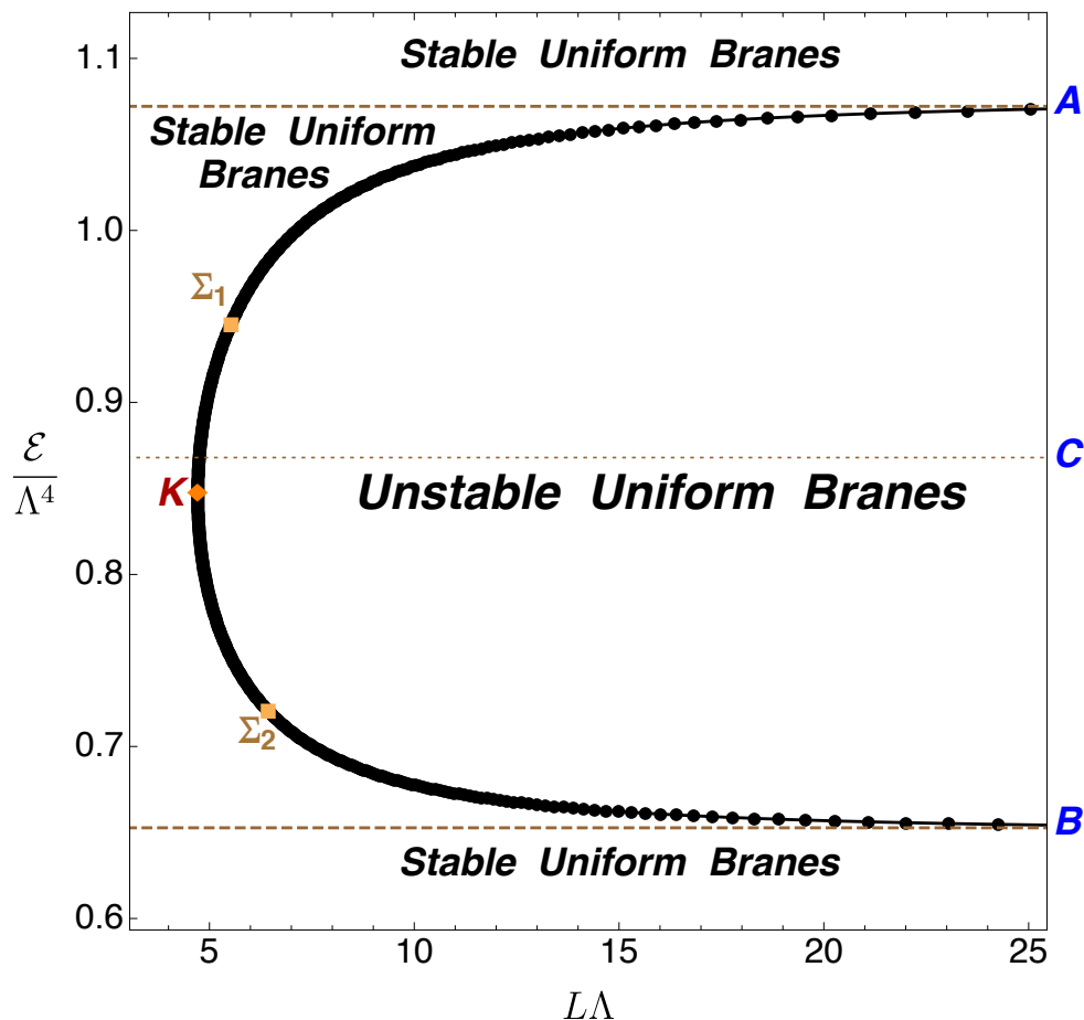
Figure 8. Stability diagram for uniform nonconformal branes. The interpretation of the two yellow square points \Sigma_1 and \Sigma_2 will be given when discussing figure 10. For reference, (\hat{T}, \hat{L}_{\text{GL}}, \hat{\mathcal{E}})_{\Sigma_1} \simeq (0.390817, 5.618133, 0.950579) and (\hat{T}, \hat{L}_{\text{GL}}, \hat{\mathcal{E}})_{\Sigma_2} \simeq (0.404645, 6.592316, 0.717060) and (\hat{T}, \hat{L}_{\text{GL}}, \hat{\mathcal{E}})_K \simeq (0.397427, 4.716021, 0.846337) .
