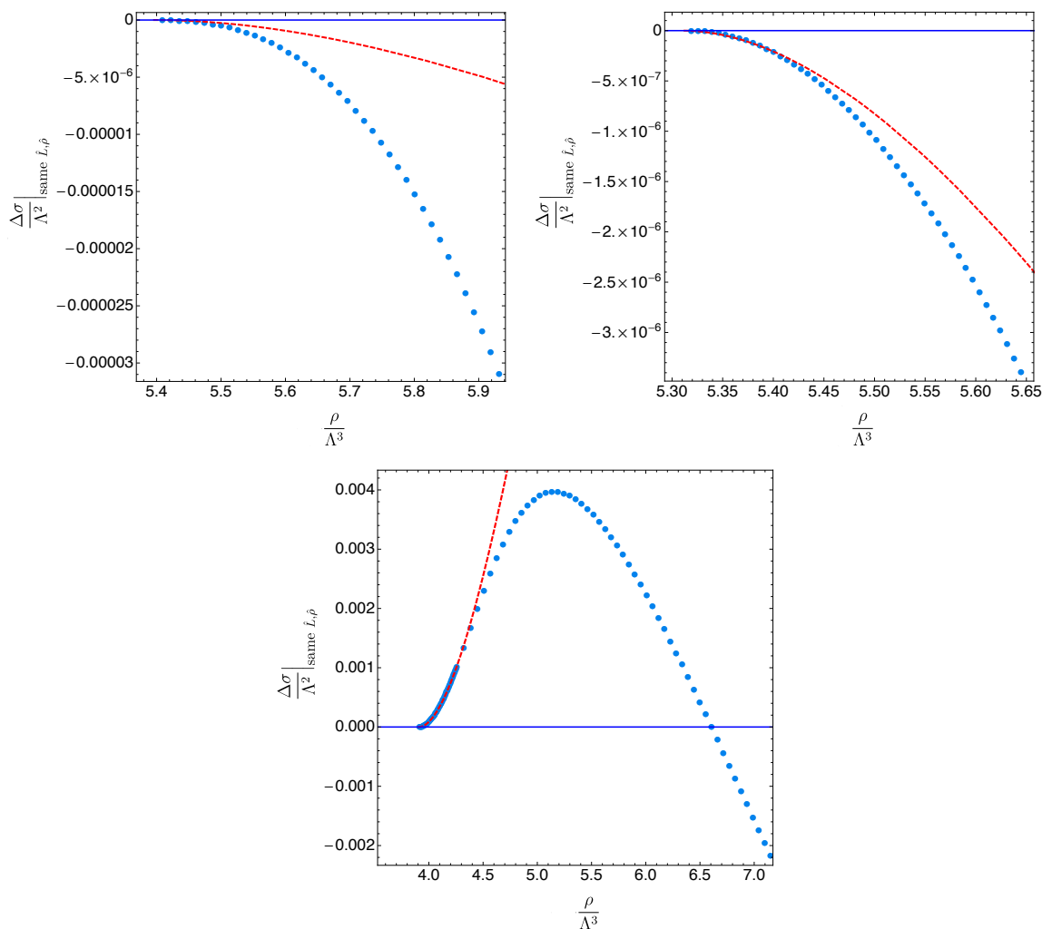
Figure 14. Difference \Delta\hat{\sigma}|_{\text{same}\hat{L},\hat{\rho}} between the Killing entropy densities of lumpy and uniform branes with the same (\hat{L}, \hat{\rho}) as a function of the Killing energy density \hat{\rho} for three constant- \hat{T} families of lumpy branes with \hat{T} \simeq 0.390711 < \hat{T}_{\Sigma_1} (top-left), \hat{T} \simeq 0.405141 > \hat{T}_{\Sigma_2} (top-right) and \hat{T}_{\Sigma_1} < \hat{T} \simeq 0.399547 < \hat{T}_{\Sigma_2} (bottom). Recall that \hat{T}_{\Sigma_1} \simeq 0.390817 and \hat{T}_{\Sigma_2} \simeq 0.404645 . The blue dots are the numerical results for the lumpy branes. The dashed, red curves are the perturbative result (2.72). The horizontal blue line indicates the uniform-brane family.
