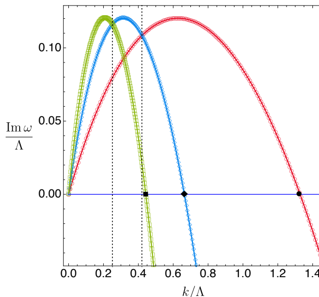
Figure 21. Dispersion relation of GL modes for a uniform brane with (\hat{\tau}, \hat{\mathcal{E}}) \simeq (0.395894, 0.867966) . Red circles, blue diamonds and green squares correspond to harmonics with \eta = 1, 2 and 3 , respectively. For reference the maximum of the instability occurs for (\hat{\tau}, \hat{k}_{\text{GL}})_K \simeq (0.397427, 1.332306) , i.e. (\hat{\tau}, \hat{L}_{\text{GL}})_K \simeq (0.397427, 4.716021) . The GL zero mode was identified in figure 7.
