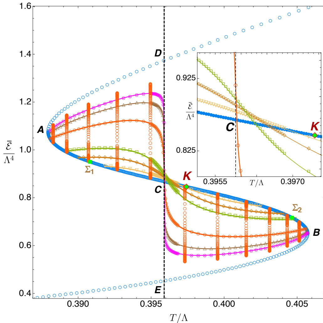
Figure 11. Phase diagram of figure 3 now with both uniform branes (blue circles) and some nonuniform brane solutions at constant temperature \hat{T} (orange circles) or constant length \hat{L} . The eleven constant-temperature vertical lines have (from left to the right): \hat{T} \simeq \{0.388292, 0.389219, 0.390711, 0.392677, 0.394948, 0.397308, 0.399547, 0.401511, 0.403112, 0.404320, 0.405141\} . The six lumpy-brane curves at constant \hat{L} have (from bottom to top on the left): \hat{L}_\nabla \simeq 5.299674 , \hat{L}_\diamond \simeq 6.004224 , \hat{L}_\square \simeq 6.900924 , \hat{L}_\circ \simeq 11.501849 , \hat{L}_\triangle \simeq 17.906849 , \hat{L}_\otimes \simeq 24.311849 . The inset plot is a zoom in around the region that contain C and K (see also figure 7) and here we plot the uniform-brane curve and just the four constant- \hat{L} curves \{\hat{L}_\nabla, \hat{L}_\diamond, \hat{L}_\square, \hat{L}_\circ\} . For reference, (\hat{T}, \hat{\mathcal{E}})_{\Sigma_1} \simeq (0.390817, 0.950579) , (\hat{T}, \hat{\mathcal{E}})_{\Sigma_2} \simeq (0.404645, 0.717060) and (\hat{T}, \hat{\mathcal{E}})_K \simeq (0.397427, 0.846337) .
