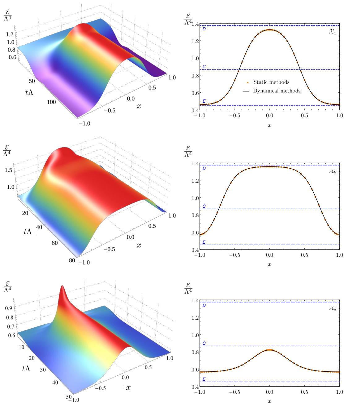
Figure 24. Real-time evolution leading to a type I (top-left), a type II (middle-left) and a type III (bottom-left) lumpy brane with \hat{L} \simeq 11.501849 , labelled \mathcal{X}_a , \mathcal{X}_b and \mathcal{X}_c in figure 22, respectively. On the right panels we compare the energy density profiles at late times (continuous black lines) with those obtained by static methods (orange dots).
