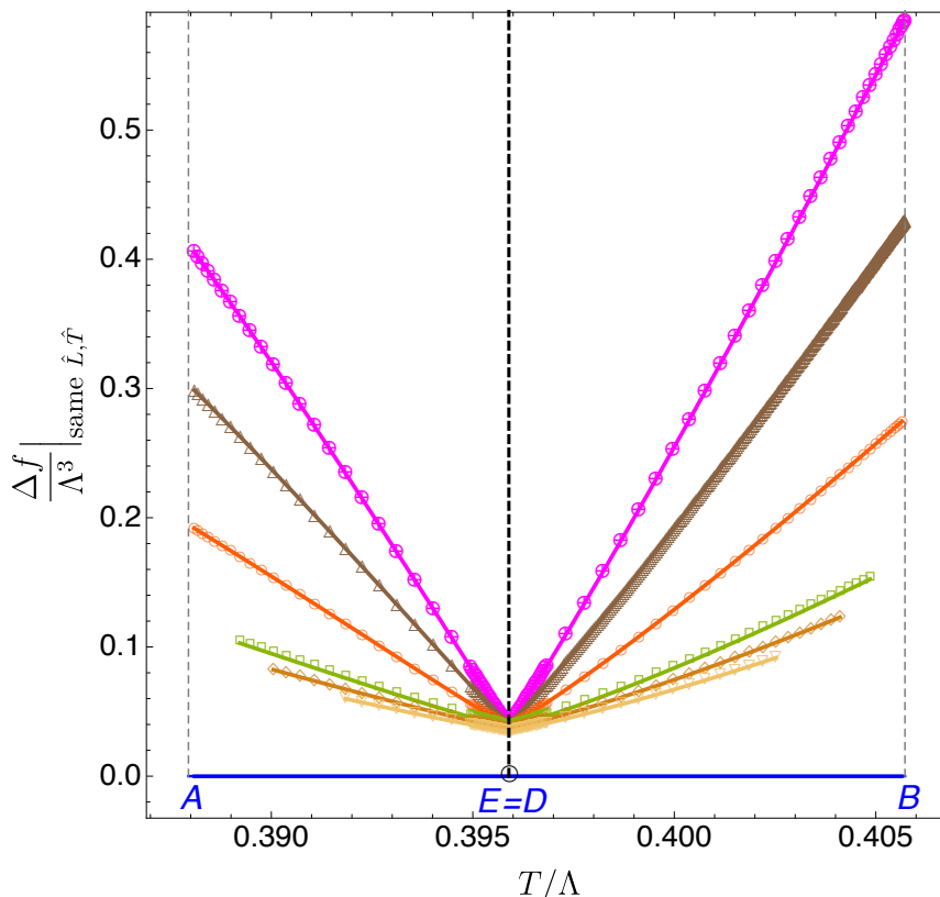
Figure 19. Canonical phase diagram: dimensionless Killing free energy density difference \Delta\hat{f}|_{\text{same}\hat{L},\hat{T}} as a function of the dimensionless temperature \hat{T} for the six lumpy-brane families at constant \hat{L} already shown in figure 11 (with the same colour/shape code). Namely, from the bottom to the top the length of the curves are: \hat{L}_\nabla \simeq 5.299674 , \hat{L}_\diamond \simeq 6.004224 , \hat{L}_\square \simeq 6.900924 , \hat{L}_\circ \simeq 11.501849 , \hat{L}_\Delta \simeq 17.906849 , \hat{L}_\otimes \simeq 24.311849 . The black dashed vertical line with \hat{T} = \hat{T}_D = \hat{T}_E \equiv \hat{T}_c \sim 0.3958945 represents the critical temperature first identified in the right panel of figure 3 and the grey vertical dashed lines represent \hat{T} = \hat{T}_A \sim 0.387944 and \hat{T} = \hat{T}_B \sim 0.405724 between which lumpy branes coexist with uniform branes. The horizontal blue line with \Delta\hat{f} = 0 represents the light uniform brane for \hat{T} < \hat{T}_c , and the heavy uniform brane for \hat{T} > \hat{T}_c .
