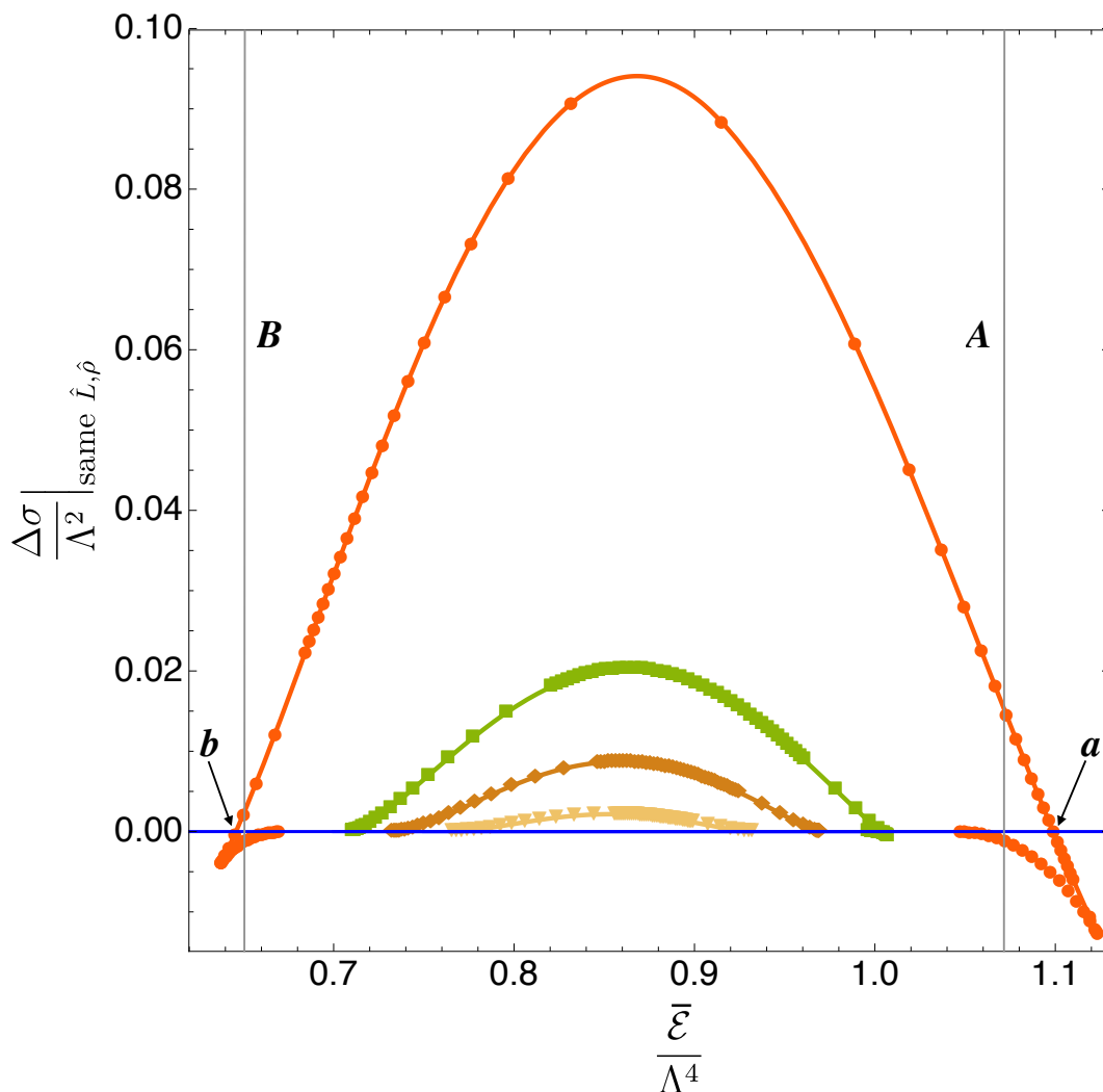
Figure 18. Killing entropy density difference \Delta\hat{\sigma}|_{\text{same}\hat{L},\hat{\rho}} between lumpy and uniform branes with the same (\hat{L},\hat{\rho}) or, equivalently, with the same (\hat{L},\hat{\mathcal{E}}) , as a function of the average energy density \hat{\mathcal{E}} . We show the same four families of lumpy branes with constant \{\hat{L}_\blacktriangledown,\hat{L}_\blacklozenge,\hat{L}_\blacksquare,\hat{L}_\bullet\} \simeq \{5.299674, 6.004224, 6.900924, 11.501849\} already displayed in figure 11. We use the same shape/colour coding for the markers as in figure 11 except that here they are all solid. The families with \blacktriangledown, \blacklozenge, \bullet were also shown in figure 17, but the family \blacksquare was not. The horizontal blue line with \Delta\hat{\sigma}|_{\text{same}\hat{L},\hat{\rho}} = 0 describes the uniform brane family. The grey vertical lines indicate the turning points A and B in the phase diagram of figure 3. The labels “ a ” and “ b ” indicate the lumpy solutions with \hat{L}_\bullet \simeq 11.501849 that lie away from the merger curve but have the same entropy density as the corresponding uniform branes. In other words, these are the points away from the merger curve at which \Delta\hat{\sigma}|_{\text{same}\hat{L},\hat{\rho}} crosses zero. The average energy densities at these points are \hat{\mathcal{E}}_a \simeq 1.09879 > \hat{\mathcal{E}}_A and \hat{\mathcal{E}}_b \simeq 0.645861 < \hat{\mathcal{E}}_B .
