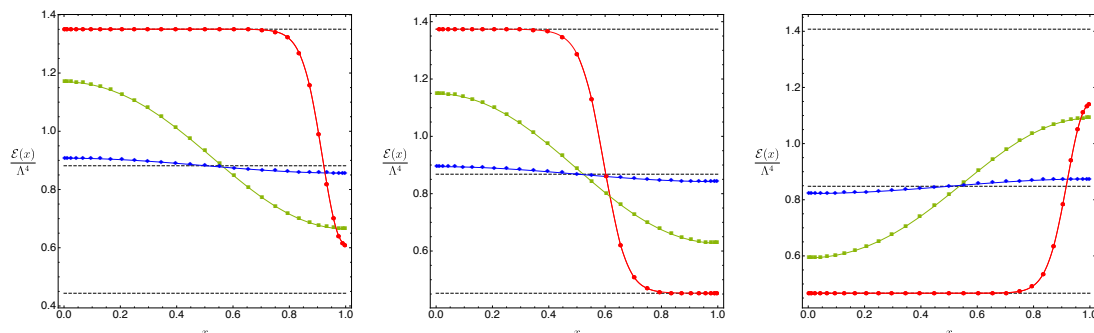
Figure 12. Energy density profile \hat{\mathcal{E}}(x) for three lumpy branes at the same temperature \hat{T} . 14 (Left) Lumpy branes at constant \hat{T} \simeq 0.394948 (this is the first vertical line of orange circles to the left of C in figure 11). For reference, at the merger the lumpy brane with this temperature has \hat{L} = \hat{L}_{\text{GL}} \simeq 4.808993 and \hat{L}_{\blacklozenge} \simeq 4.819793 , \hat{L}_{\blacksquare} \simeq 5.996993 , \hat{L}_{\bullet} \simeq 37.208993 . For this temperature the heavy, intermediate and light uniform branes have energy densities \hat{\mathcal{E}}^{\text{heavy}} \simeq 1.350615 , \hat{\mathcal{E}}^{\text{inter}} \simeq 0.881537 and \hat{\mathcal{E}}^{\text{light}} \simeq 0.443756 , respectively. These energy densities are indicated by the dashed horizontal lines in the plot. (Middle) Lumpy branes at constant \hat{T} \simeq 0.395894 \lesssim \hat{T}_c (so, very close to \hat{T}_c \simeq 0.3958945 ). For reference, \hat{L} = \hat{L}_{\text{GL}} \simeq 4.750995 and \hat{L}_{\blacklozenge} \simeq 4.761845 , \hat{L}_{\blacksquare} \simeq 5.944495 , \hat{L}_{\bullet} \simeq 46.523495 , and the energy densities of the relevant uniform branes (dashed horizontal lines) are \hat{\mathcal{E}}^{\text{heavy}} \simeq 1.373843 , \hat{\mathcal{E}}^{\text{inter}} \simeq 0.867966 , \hat{\mathcal{E}}^{\text{light}} \simeq 0.452747 . (Right) Lumpy branes at constant \hat{T} \simeq 0.397308 (this is the first vertical line of orange circles to the right of C in figure 11). For reference, at the merger the lumpy brane with this temperature has \hat{L} = \hat{L}_{\text{GL}} \simeq 4.716232 and \hat{L}_{\blacklozenge} \simeq 4.727157 , \hat{L}_{\blacksquare} \simeq 5.917982 , \hat{L}_{\bullet} \simeq 34.759982 , and the energy densities of the relevant uniform branes (dashed horizontal lines) are \hat{\mathcal{E}}^{\text{heavy}} \simeq 1.407521 , \hat{\mathcal{E}}^{\text{inter}} \simeq 0.848014 , \hat{\mathcal{E}}^{\text{light}} \simeq 0.467119 .
