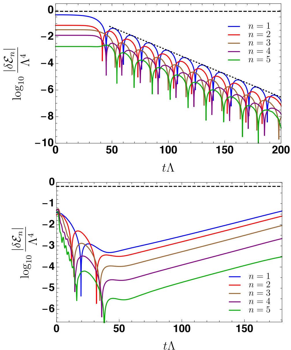
Figure 25. (Top) Time evolution of some Fourier modes of a perturbation around the type I, inhomogeneous, static configuration \mathcal{X}_a of figure 24(top-right) with \hat{\mathcal{E}} \simeq 0.831460 , \hat{L} \simeq 11.501849 . The dashed horizontal line indicates the average energy density of the box. The region with clear exponentially damped oscillations corresponds to times where the subdominant modes have decayed sufficiently, and the dominant mode has leading amplitude. The dotted line corresponds to a fit to the envelope, from which we extract the imaginary part of \omega . The fact that no mode grows in time indicates that \mathcal{X}_a is locally dynamically stable. (Bottom) Time evolution of some Fourier modes of a perturbation around the type III, inhomogeneous, static configuration \mathcal{X}_c of figure 24(bottom-right) with \hat{\mathcal{E}} \simeq 0.651 , \hat{L} \simeq 11.501849 . In this case the leading mode grows exponentially in time, indicating that \mathcal{X}_c is locally dynamically unstable.
