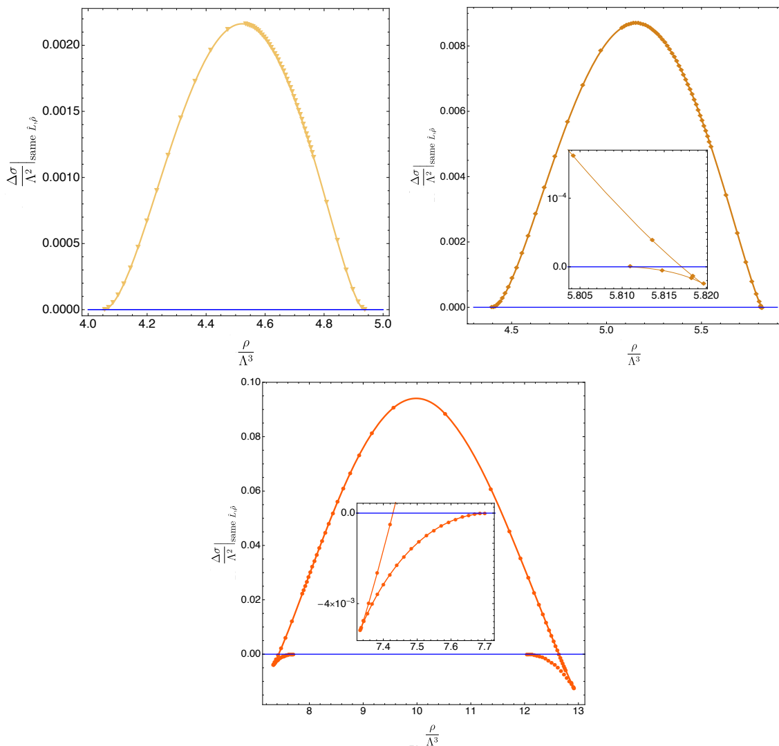
Figure 17. Microcanonical phase diagram: Killing entropy density difference \Delta\hat{\sigma}|_{\text{same}\hat{L},\hat{\rho}} between lumpy and uniform branes with the same (\hat{L},\hat{\rho}) as a function of the Killing energy density \hat{\rho} for 3 families of lumpy branes that have constant \hat{L} given by \hat{L} \simeq 5.299674 < \hat{L}_{\Sigma_1} (top-left), \hat{L} \simeq 6.004224 which is in the range \hat{L}_{\Sigma_1} < \hat{L} < \hat{L}_{\Sigma_2} (top-right) and \hat{L} \simeq 11.501849 > \hat{L}_{\Sigma_2} (bottom). For reference, \hat{L}_{\Sigma_1} \simeq 5.618133 and \hat{L}_{\Sigma_2} \simeq 6.592316 . The three families are those with constant \{\hat{L}_\blacktriangledown, \hat{L}_\blacklozenge, \hat{L}_\bullet\} already displayed in figure 11; we use the same shape/colour coding for the markers except that here they are all solid. The horizontal blue line with \Delta\hat{\sigma}|_{\text{same}\hat{L},\hat{\rho}} = 0 describes the uniform brane family.
