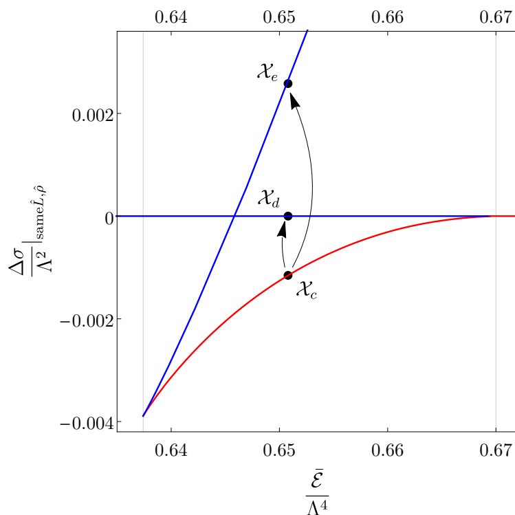
Figure 27. Zoom-in on the left region of figure 22, where \hat{L} \simeq 11.501849 . \mathcal{X}_c , \mathcal{X}_d and \mathcal{X}_e are the three static solutions with the same average energy density \hat{\mathcal{E}} \simeq 0.651 . The nonlinear time evolution of figure 28(left) corresponds to an evolution from \mathcal{X}_c to \mathcal{X}_d , and figure 28(right) corresponds to an evolution from \mathcal{X}_c to \mathcal{X}_e .
