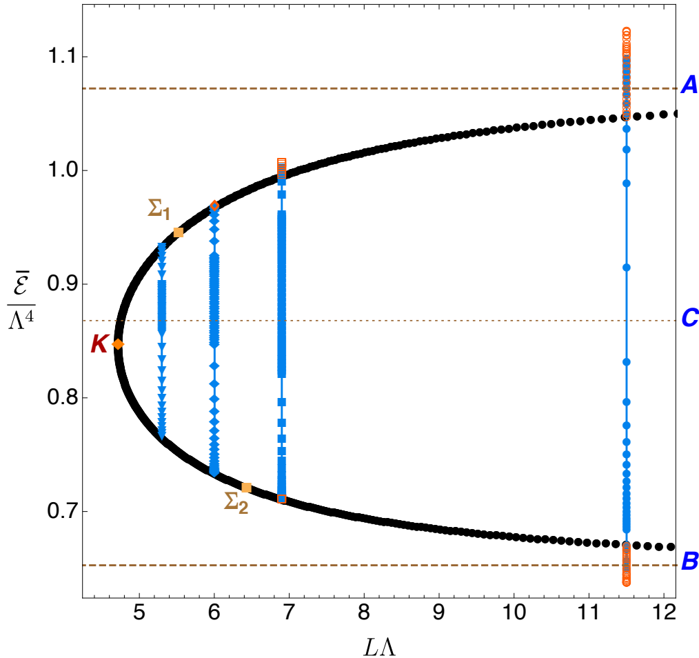
Figure 16. Same stability diagram as in figure 8 with the inclusion of some lumpy-brane lines that bifurcate from the GL merger curve. These lines have constant \hat{L} given by \{\hat{L}_\blacktriangledown, \hat{L}_\blacklozenge, \hat{L}_\blacksquare, \hat{L}_\bullet\} \simeq \{5.299674, 6.004224, 6.900924, 11.501849\} . Solid blue markers (empty orange markers), no matter their shape, indicate positive (negative) \Delta\hat{\sigma}|_{\text{same}\hat{L},\hat{\rho}} . Note that some orange circles are on top of some blue disks. This describes the region around the cusps of figure 17 and 18.
