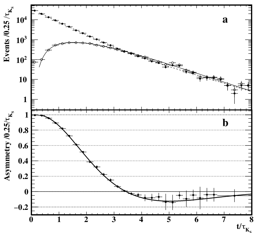
Figure 6. (a) “Toy” MC generated time-dependent decay rates. The histogram with filled black circles corresponds to “right sign” and with open circles correspond to the “wrong sign” decay rates. The solid and dashed lines correspond to the result of the simultaneous fit. (b) The resulting decay rate asymmetry with the fit result superimposed.
