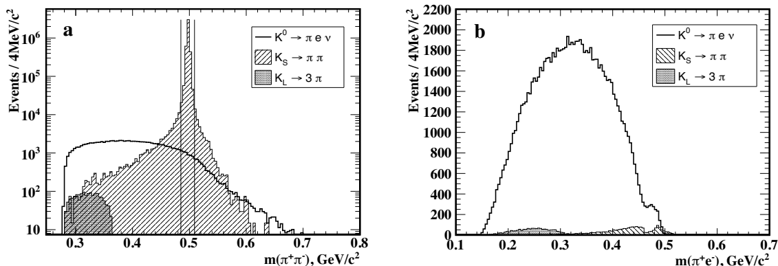
Figure 4. (a) Distribution of the \pi^+\pi^- invariant mass. The contributions from three processes are drawn. Here the pion mass is also assigned to an electron from K^0 \rightarrow \pi e \nu decay. The vertical lines show the proposed K_S^0 veto. Applying this veto one can obtain the e\pi invariant mass distribution shown in the right (b) where hatched histograms represent the background contribution.
