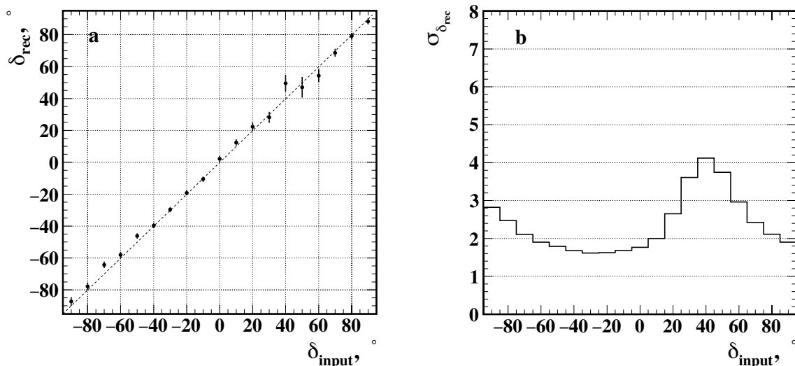
Figure 7. (a) Resulting \delta values extracted from the fit with the obtained uncertainty (b).
