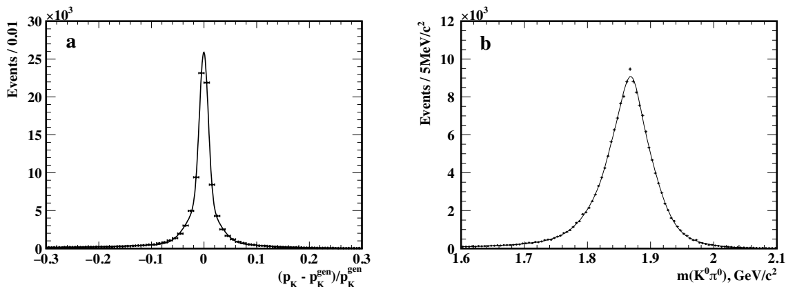
Figure 3. (a) Relative K^0 momentum resolution, (b) distribution of the K^0\pi^0 invariant mass for selected candidates.
