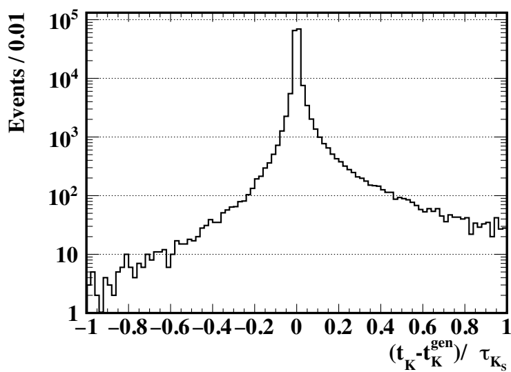
Figure 5. Resulting kaon lifetime resolution.
