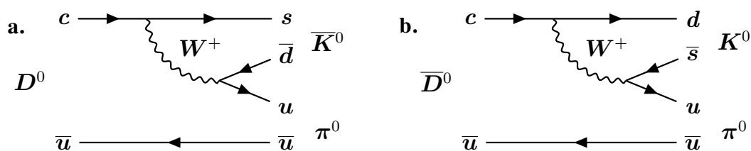
Figure 1. Feynman diagrams for (a) CF and (b) DCS D^0 \rightarrow \bar{K}^0 \pi^0 decays.
