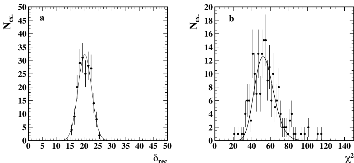
Figure 8. (a) Distribution of \delta values obtained in 200 pseudoexperiments and (b) distribution of chi-square values. The solid lines are fit results with Gaussian and chi-square distribution functions, respectively.
