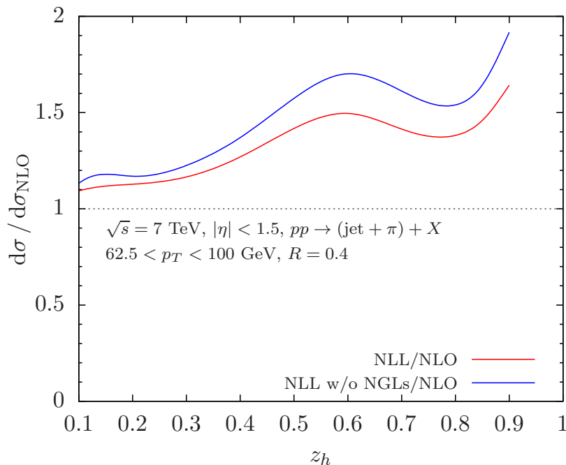
Figure 4. Ratio of the threshold resummed cross section and the NLO with (red) and without (blue) NGLs. The kinematics are the same as in figure 1.
