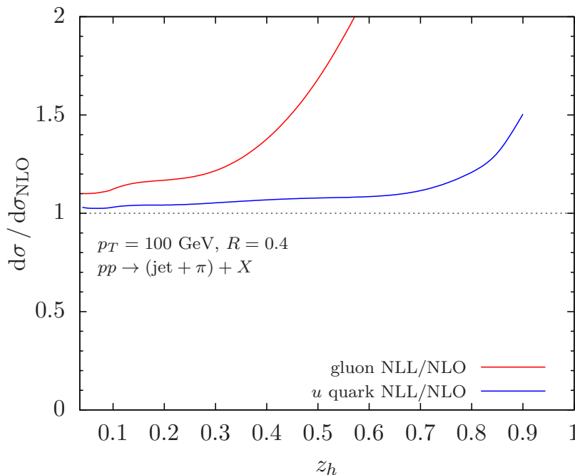
Figure 2. Ratio of the threshold resummed and the NLO cross section for the gluon (red) and the u quark jet function (blue). The kinematics are the same as in figure 1.
