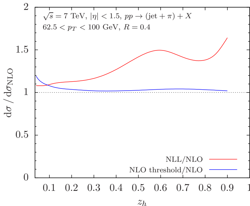
Figure 1. Ratio of the threshold resummed and the NLO cross section (red) for the longitudinal momentum distribution z_h of pions inside a jet pp \rightarrow (\text{jet} + \pi) + X . The kinematics are indicated in the figure and we use the pion fragmentation functions of [15]. In addition, we show in blue the ratio of the NLO cross section in the threshold limit and the full NLO.
