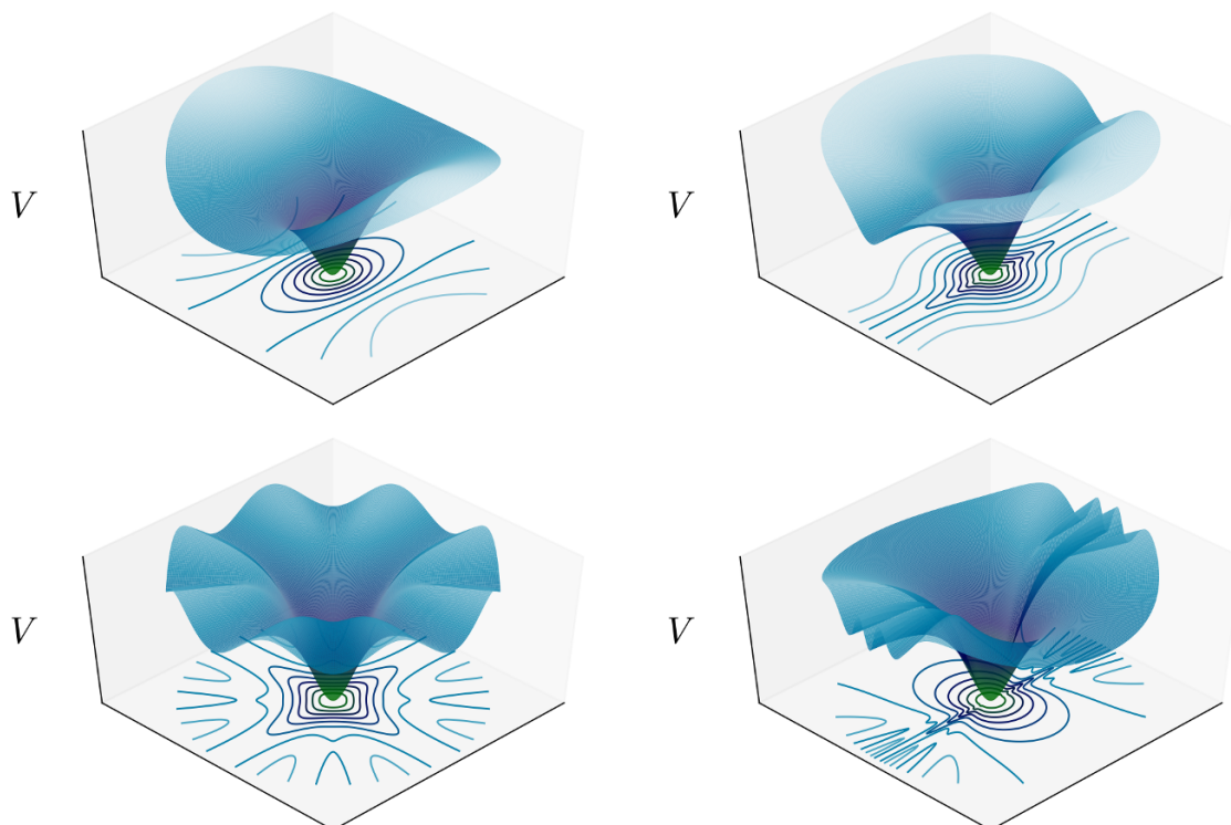
Figure 1. Potential for the N = 2 case plotted in the polar coordinates \{\varphi, \psi\} , with angles \theta_1 and \theta_2 minimized. The top-left plot shows the potential eq. (3.7) up to terms with p = 1 , in the case of equal A_i . The top-right plot shows the same potential but for A_1 = 1 and A_2 = 0.2 . The bottom-left plot shows the potential with terms up to p = 4 , in the case of equal A_i . The bottom-right plot shows the same potential but for A_1 = 1 and A_2 = 0.2 . We can see that the elliptical structure of the model makes valleys in the potential bundle-up. While different radial directions have plateaus with different amplitudes, the exponential fall-off has the same signature for all initial conditions, or in other words, values of the angular coordinate \psi_\beta . The oscillating plateau of the circular case were already noted for a real 2-disk \alpha -attractor (without supergravity) in [48].
