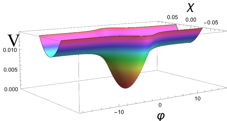
Figure 4. Inflaton potential of the T-model version of the fibre inflation potential for a particular case M = m = 0.1 , \mathcal{V}_0 = 2\sqrt{2} .
