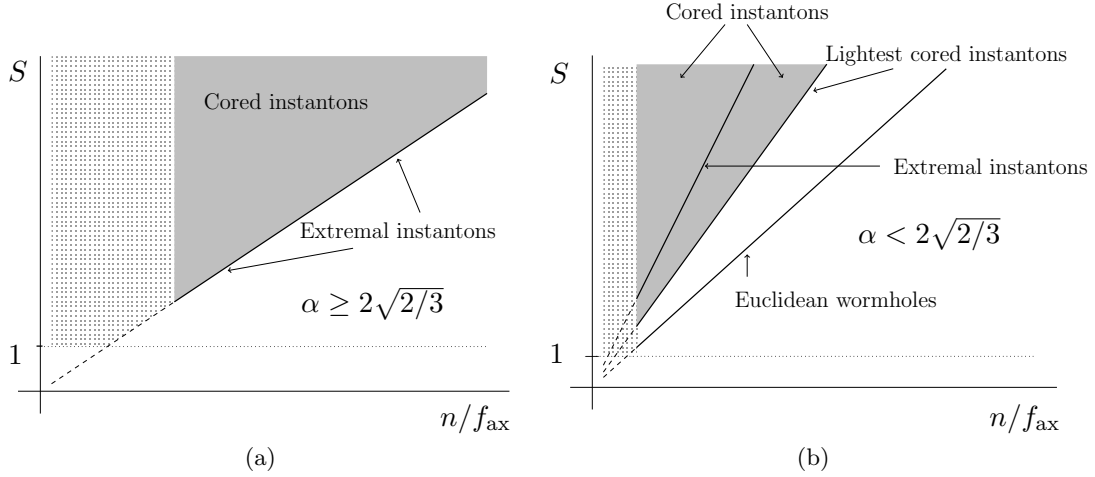
Figure 9. Instanton action S vs. n/f_{\text{ax}} for (a) \alpha \geq 2\sqrt{2/3} and (b) \alpha < 2\sqrt{2/3} .
