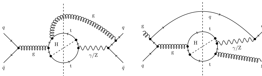
Figure 3. Two Feynman diagrams squared for real corrections featuring interference between QCD and EW tree-level diagrams. The decay products of the top quarks are not shown as their inclusion does not alter the discussion.
