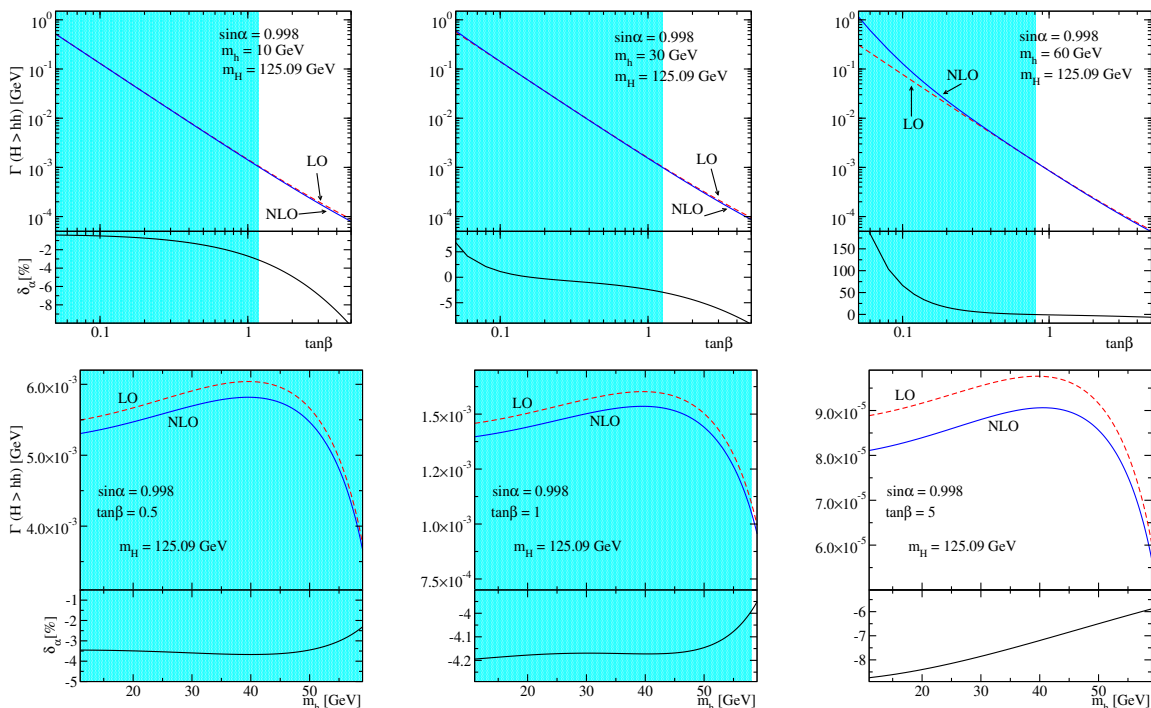
Figure 8. Heavy-to-light Higgs boson width \Gamma_{H\rightarrow hh} in the low-mass region. The results are shown at LO (dashed, red) and NLO (full, blue) as a function of the relevant parameters of the model. The mixing angle is fixed to \sin\alpha = 0.998 in all cases. The lower subpanels show the relative EW one-loop correction in the \alpha_{em} -parametrization (4.7). Renormalization is performed in the improved on-shell scheme. The shaded areas in the low \tan\beta and m_h ranges are ruled out by the LHC Higgs signal strength measurements.
