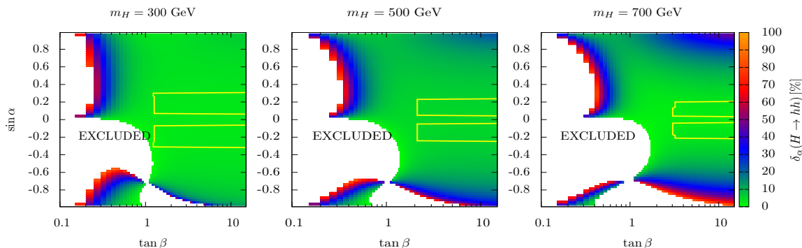
Figure 5. Relative one-loop EW corrections in the \alpha_{\text{em}} -parametrization (4.7), projected on the \sin \alpha - \tan \beta plane for exemplary heavy Higgs masses in the high-mass region. The white voids correspond to regions with \delta_\alpha \gtrsim 100\% . Renormalization is performed in the improved on-shell scheme. The yellow contour separates the allowed and excluded regions in the parameter space.
