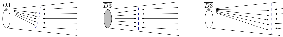
Figure 2. The “gluing surface” between the near- \overline{D3} solution and the KS background is different for localized (left) and smeared sources (center). On the other hand, for a large Schwarzschild radius (right), the surface is once again SU(2) \times SU(2) invariant and the mass parameters are independent of the anti-branes position at the tip.
