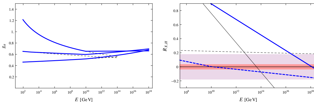
Figure 2. Intermediate scale supersymmetry breaking with TeV-scale wino. Caption as in figure 1, except both shaded (red) bands have been drawn for V/\Lambda = 0.2 .
