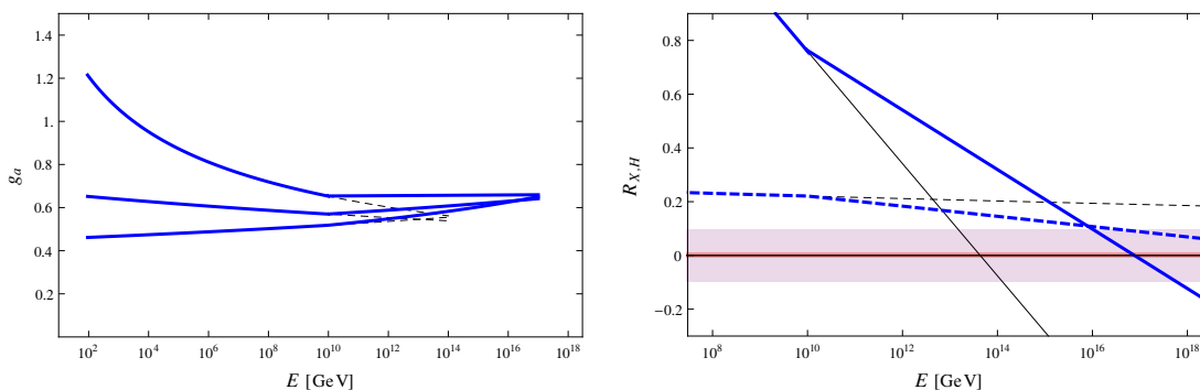
Figure 1. Pure intermediate scale supersymmetry breaking. Left panel: evolution of gauge couplings in ISS (solid, blue) and in the SM (dashed, black). Right panel: evolution of R_X (solid) and R_H (dashed) for ISS (thick, blue) and the SM (thin, black). Without corrections from dimension 5 and 6 operators, M_X and M_H are the scales at which R_X and R_H vanish, respectively. Including the dimension 5 operator, allowed values of M_H occur when the dashed thick (blue) line lies inside the pale (red) shaded region. Including the dimension 6 operators, allowed values of M_X occur when the solid thick (blue) line lies inside the dark (red) shaded region. Both shaded (red) bands have been drawn for V/\Lambda = 0.1 .
