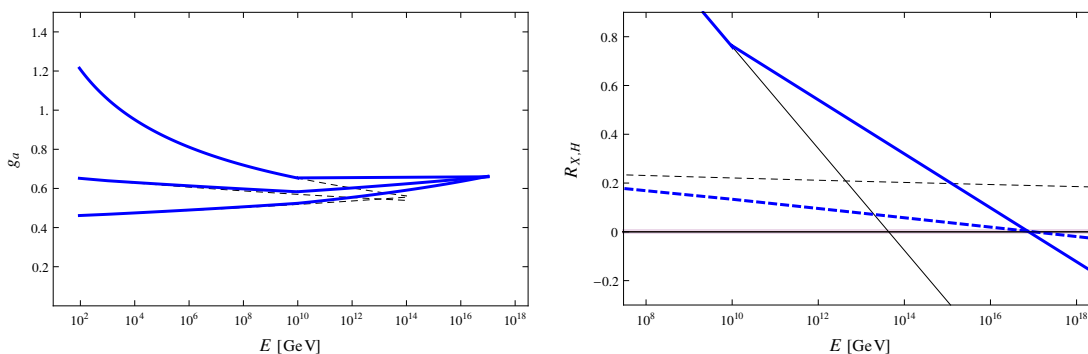
Figure 3. Intermediate scale supersymmetry breaking with TeV-scale Higgsino. Caption as in figure 1, except both shaded (red) bands have been drawn for V/\Lambda = 0.01 .
