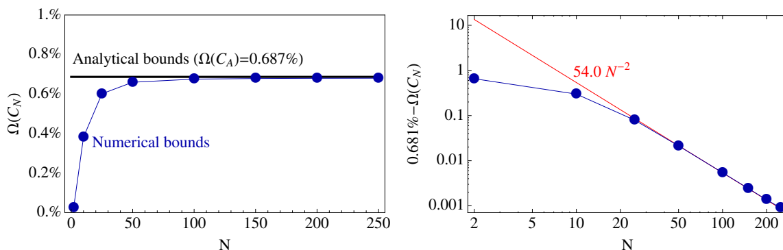
Figure 5. Solid angle \Omega(C_N) for different N values.
