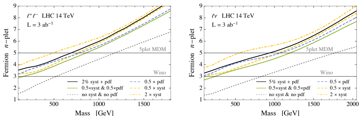
Figure 4. Dependence of the 95% CL exclusion bounds on Majorana fermion multiplets at the HL-LHC on the PDF uncertainties and on the additional systematic errors. The left and right panels show the bounds from the \ell^+\ell^- and \ell\nu channels respectively. The solid black lines give the bounds for our benchmark systematic errors. The dashed (dot-dashed) yellow lines show how the bound changes if the additional systematic uncertainties are halved (doubled). The dashed blue lines show how the bounds are modified by halving the PDF uncertainty. The solid green lines give the bound with all systematic uncertainties halved. Finally the dotted grey lines correspond to the bounds with no systematic and PDF errors.
