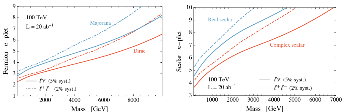
Figure 6. Expected 95% CL exclusion limits obtained for the FCC-100.
