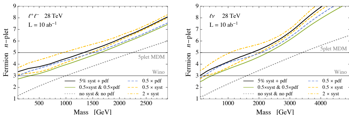
Figure 11. Dependence of the 95% CL exclusion bounds on Majorana fermion multiplets at the HE-LHC on the PDF uncertainties and on the additional systematic errors.
