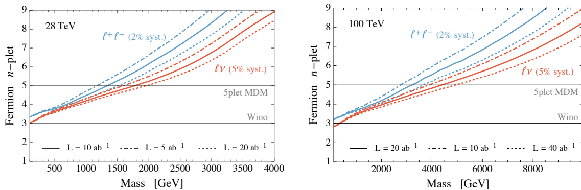
Figure 10. Dependence of the 95% CL exclusion bounds on the integrated luminosity at the HE-LHC (left panel) and at the FCC-100 (right panel). The red and blue lines correspond to the bounds from the \ell\nu and \ell^+\ell^- final states.
