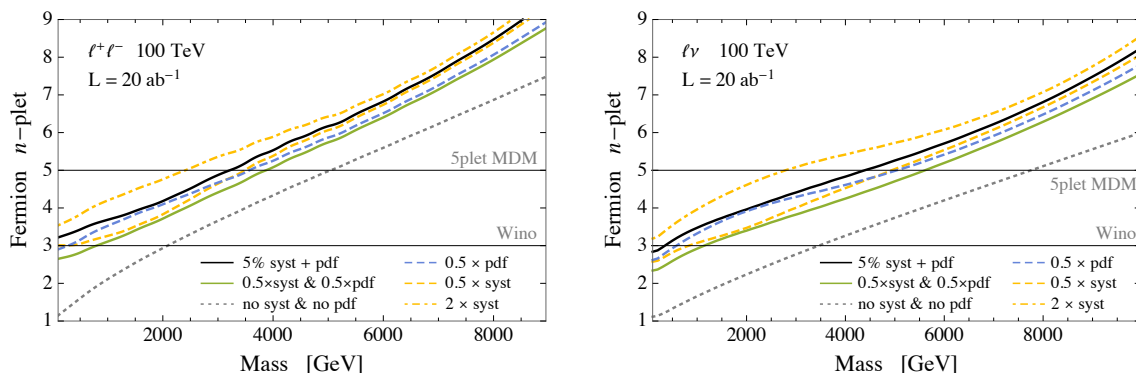
Figure 12. Dependence of the 95% CL exclusion bounds on Majorana fermion multiplets at the FCC-100 on the PDF uncertainties and on the additional systematic errors.
