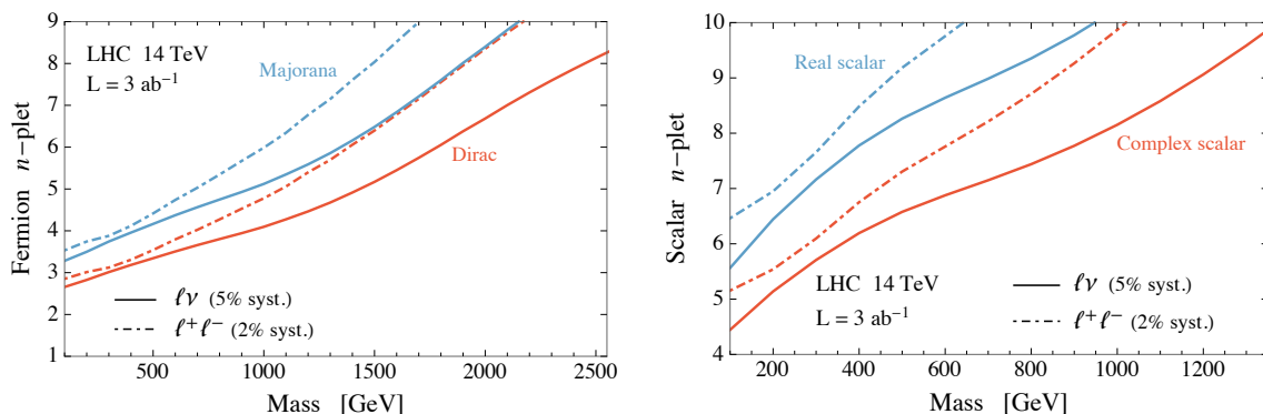
Figure 2. Expected 95% CL exclusion limits at the HL-LHC. The left and right panels show the bounds on fermion and scalar multiplets respectively. The vertical axis reports the effective n of the multiplet, while the horizontal axis gives the mass of the states in the multiplet, which are assumed to be (almost) degenerate. The solid and dot-dashed lines correspond to the bounds from the \ell\nu and \ell^+\ell^- channels respectively. The blue (red) lines give the bounds for Majorana (Dirac) fermions on the left panel and for real (complex) scalars in the right panel.
