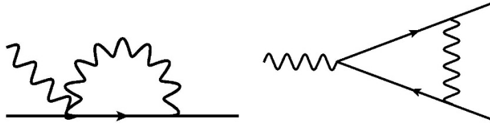
Figure 11. Two diagrams contribute to the running of the three-point vertex. Each diagram is understood to exist in several versions, with \partial_t R_k inserted on each of the internal lines in turn, such that each loop integral is UV finite.
