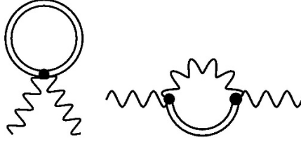
Figure 2. Double lines denote metric fluctuations and wavy lines gauge bosons. Two diagrams with quantum gravity contributions enter the expression for \eta_A .
