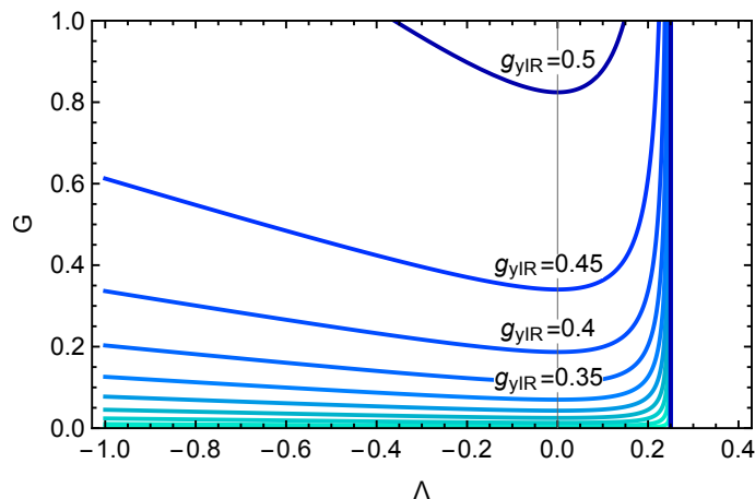
Figure 6. Lines of constant IR values of g_Y in a zoom in the region around \Lambda \approx 0 for vanishing anomalous dimension of the metric \eta_h = 0 . Within our truncation, lines of different IR values of g_Y are pulled closer together as \Lambda approaches the critical value at which the interacting fixed point merges with the free one. This moves the phenomenologically preferred values of G to significantly smaller values.
