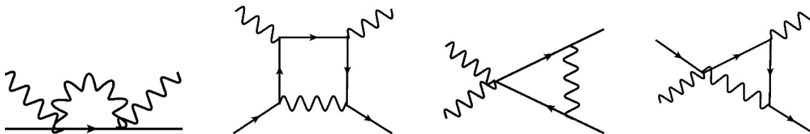
Figure 13. Four diagrams contribute to the running of the four-point vertex.
