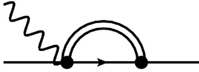
Figure 7. We show the only diagram that contributes to \beta_{\rho_3} and contains metric fluctuations. Other diagrams with internal metric fluctuations and the correct number of external legs vanish when projected onto \rho_3 according to eq. (C.1).
