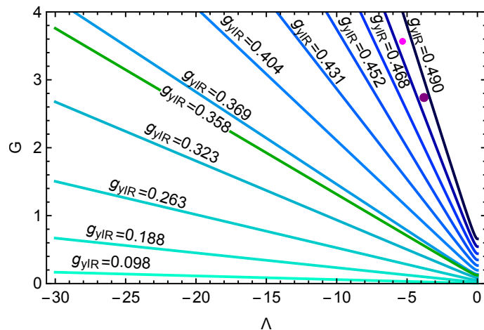
Figure 5. Lines of constant IR values for g_Y . The value extracted from measurements is highlighted in green, at g_Y = 0.358 . The larger purple dot is the fixed point obtained from eq. (4.10) with Standard Model matter content, whereas the smaller magenta dot includes the effect of three additional Weyl fermions that are required to accommodate neutrino masses. To obtain the IR values, we use that g_Y(k = M_{\text{Pl}}) = g_Y^* and use the one-loop beta function eq. (4.5) with G = 0 to integrate the flow from the Planck scale to the IR scale. The structural similarity to the dependence of the IR value of the top mass on the microscopic gravity parameters [1] is due to a similar form of the beta functions, with the only difference being the numerical prefactor of the gravity contribution as well as the critical value of \Lambda , at which the critical exponent switches its sign and an interacting, predictive fixed point is induced.
