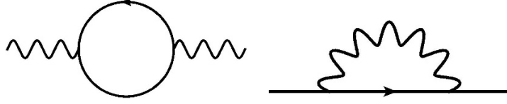
Figure 12. Diagrams contributing to the flow of the anomalous dimension \eta_A (left) and \eta_\phi (right).
