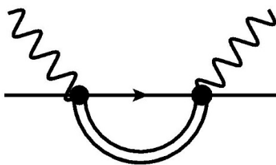
Figure 8. We show the only diagram that contributes to \beta_{\rho_4} and contains metric fluctuations. Other diagrams with internal metric fluctuations and the correct number of external legs vanish when projected onto \rho_4 according to eq. (C.12).
