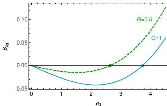
Figure 3. The beta-function for \rho exhibits an asymptotically safe fixed point under the impact of quantum gravity, cf. eq. (3.15) that depends on the microscopic values of the gravity parameters. Here we set \eta_h = 0 , \Lambda = -6 .
