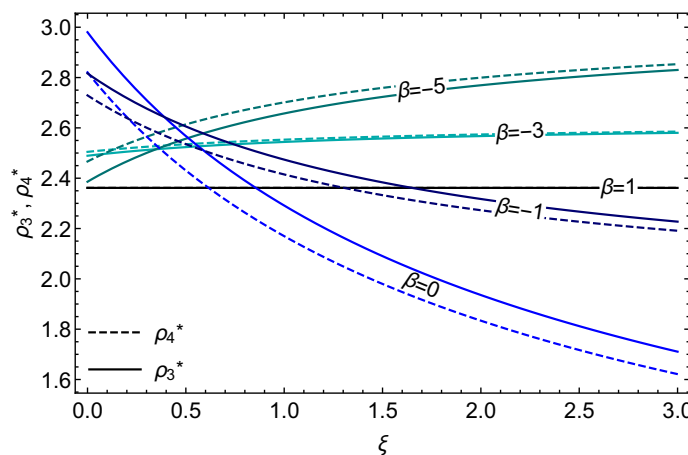
Figure 10. The interacting fixed points, \rho_{3/4}^* , as a function of the U(1) gauge parameter, \xi , for different values of the graviton gauge parameter \beta . Here \Lambda = 0 , G = 1 , \alpha = 0 .
