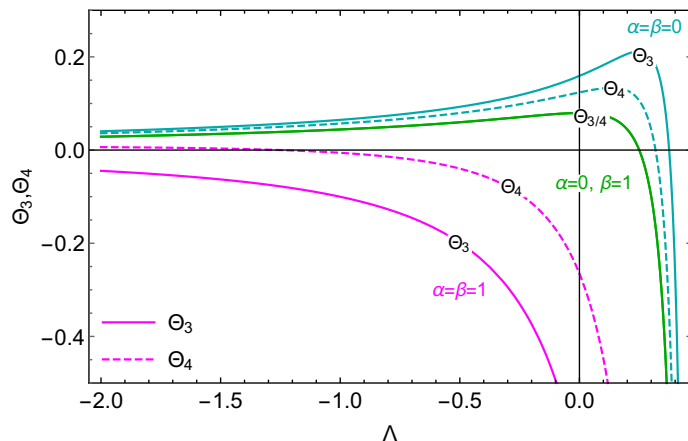
Figure 9. Critical exponent as a function of \Lambda for different gauges and G = 1 . The solid and dashed lines correspond to \Theta_3 and \Theta_4 , respectively.
