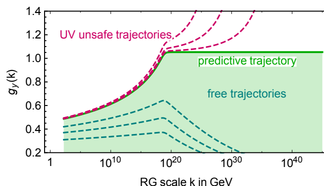
Figure 1. We show the upper bound on the IR value of g_Y under the impact of running gravitational couplings, which show a rapid transition from a classical regime below the Planck scale to a fixed-point regime above the Planck scale.
