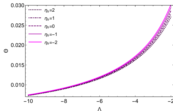
Figure 4. Significantly different choices of \eta_h , parameterizing effects beyond our truncation, only lead to slight quantitative changes of the critical exponent \Theta in the regime \Lambda < -1 that we focus on in section 4.
