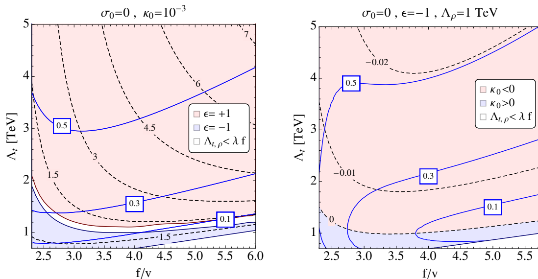
Figure 4. The solid blue lines in both plots indicate the gain in fine-tuning of the hard-breaking model with respect to the soft one. In the white region \Lambda_t < \lambda f or \Lambda_\rho < \lambda f with \lambda = 1 . Left: we take \kappa_0 = 10^{-3} and the black dashed contours show the \epsilon \times \Lambda_\rho (in TeV units) adjusted to obtain m_h = 125 GeV. The light red/blue region is the allowed parameters space with \epsilon = \pm 1 . Right: we fix \epsilon = -1 and \Lambda_\rho = 1 TeV and fix \kappa_0 (black dashed contours) to get m_h = 125 GeV. The light red/blue region is the allowed parameters space with \kappa_0 \leq 0 .
