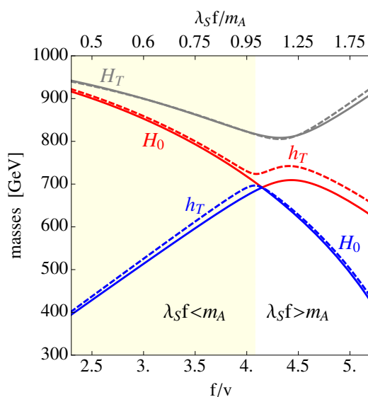
Figure 14. Left: mass eigenvalues as a function of f/v . We fix \tan\beta = 1.2 , m_{A_T} = 1 TeV and \lambda_S = 1 . The solid lines are obtained using the analytic expressions in eq. (B.14) in the v \rightarrow 0 limit. The dashed lines are obtained numerically including v/f corrections. The light yellow/white area correspond to the region where \lambda_S f \leq m_A as indicated in the plot.
