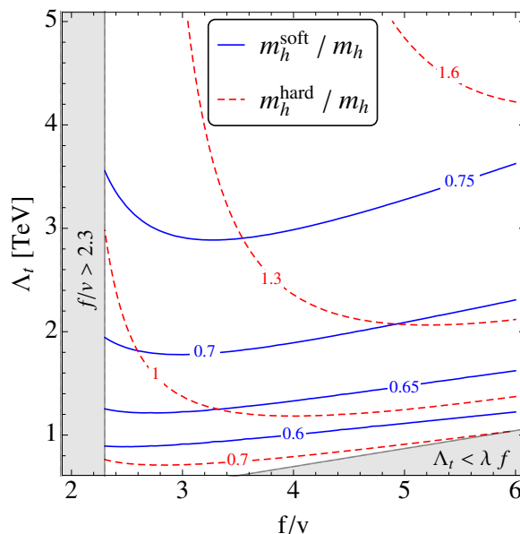
Figure 2. The blue contours indicate the irreducible contributions to the Higgs mass in the pure soft breaking scenario ( \rho_0 = 0 ), coming from top loops normalized to m_h = 125 GeV. The red dashed contours indicate the irreducible contributions to the Higgs mass in the pure hard breaking case ( \sigma_0 = 0 ), where we fix \lambda = 1 , \Lambda_\rho = 1 TeV and \epsilon = +1 in eqs. (2.5) and (2.7). The grey shaded region at the left edge with f < 2.3v is excluded by Higgs coupling measurements and the grey region at the bottom right of the plot has \Lambda_t < \lambda f .
