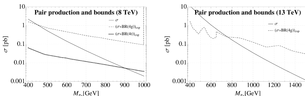
Figure 8. Color octet pair production cross section (from ref. [59]) and the current bounds on \sigma \times BR(pp \rightarrow \bar{t}t) [109, 110] and \sigma \times BR(pp \rightarrow 4j) [107] for \sqrt{s} = 8 TeV (left) and \sigma \times BR(pp \rightarrow 4j) [108] for \sqrt{s} = 13 TeV (right).
