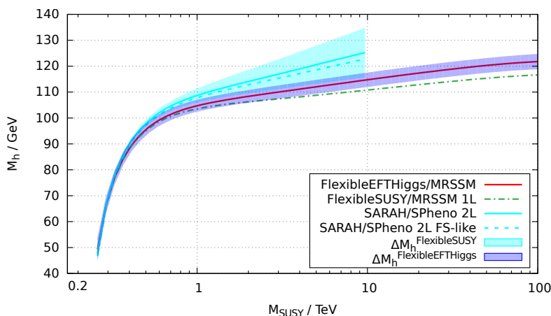
Figure 15. Predictions for M_h and combined theoretical uncertainty estimates for FlexibleSUSY and FlexibleEFTHiggs in the MRSSM, compared with results of other codes as a function of M_{\text{SUSY}} for the parameter point specified in eqs. (7.6).
