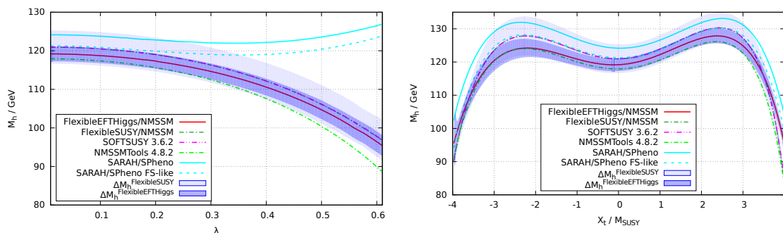
Figure 11. As figure 10, but for other parameter choices. We fix M_{\text{SUSY}} = 10 \text{ TeV} and \tan\beta = 5 and plot M_h against i) (left panel) \lambda , where \kappa = \lambda , X_t = 0 and ii) (right panel) X_t where \kappa = \lambda = 0.01 .
