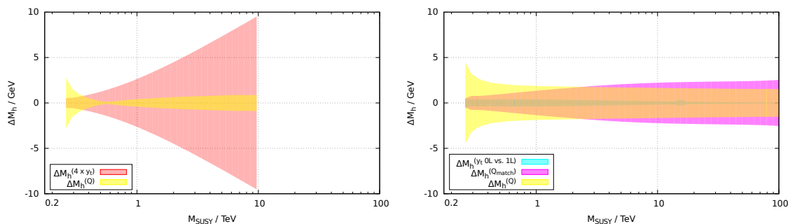
Figure 14. Uncertainty estimates of section 3 for M_h , applied to the fixed-order approach with SARAH/SPheno (left panel) and to FlexibleEFTHiggs/MRSSM (right panel) as a function of M_{\text{SUSY}} for the MRSSM parameter point (7.6).
