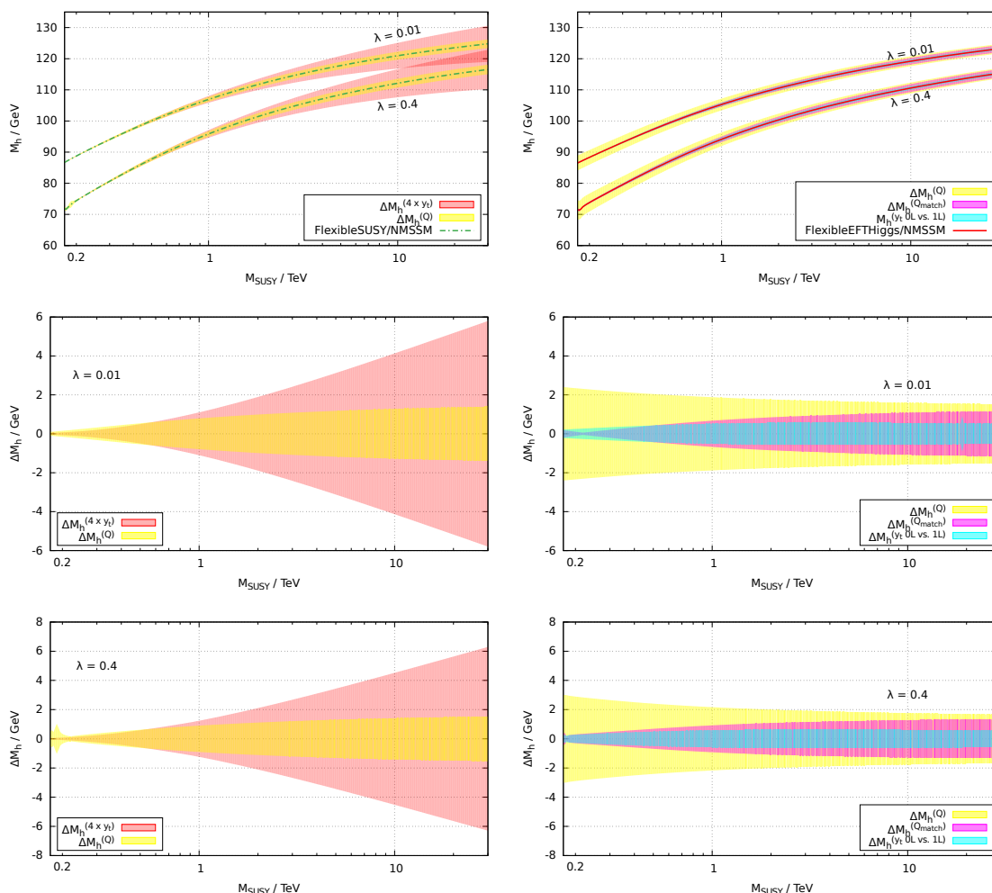
Figure 9. Higgs mass predictions and uncertainty estimates of section 3 applied to the fixed-order calculations with FlexibleSUSY and to FlexibleEFTHiggs in the NMSSM. The top row shows the Higgs mass predictions and the uncertainty estimates, the lower two rows only the uncertainty estimates, as in figure 7. The values of the singlet Yukawa couplings are \kappa = \lambda = 0.01 or \kappa = \lambda = 0.4 , as indicated in the plots. In all panels we have fixed X_t = 0 and \tan \beta = 5 .
