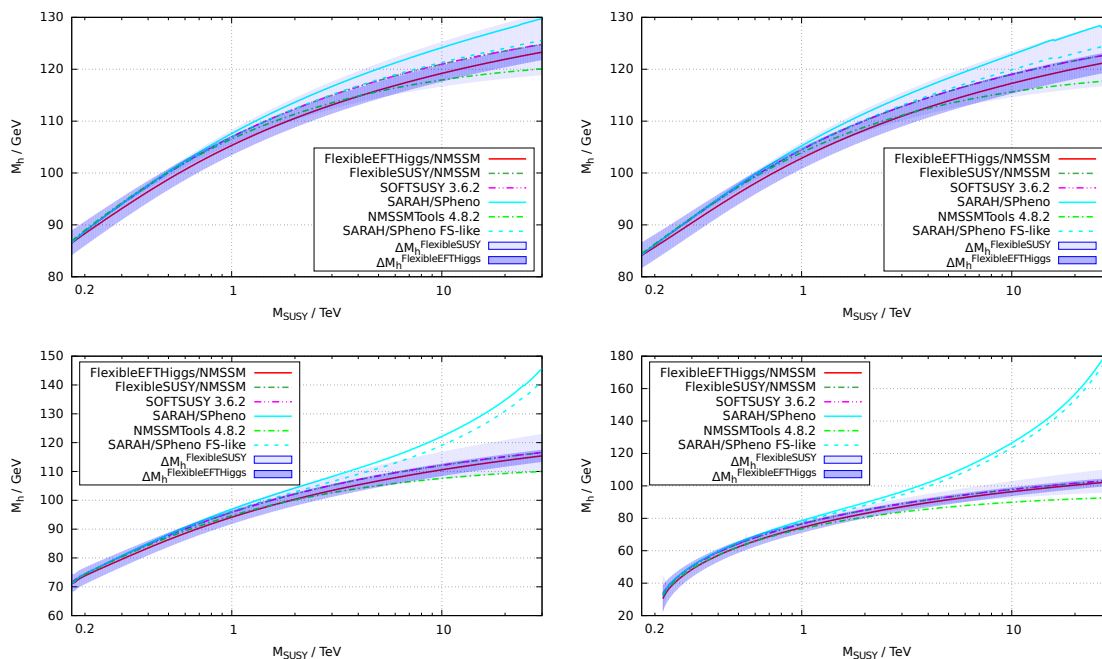
Figure 10. Predictions for M_h and combined theoretical uncertainty estimates for FlexibleSUSY and FlexibleEFTHiggs in the NMSSM, compared with results of other codes. We choose X_t = 0 and \tan\beta = 5 in all panels. The top panel shows \lambda = \kappa = 0.01 (left), which is close to the MSSM limit and \lambda = \kappa = 0.2 (right). In both cases the situation is quite similar to the MSSM. Row 2 shows \lambda = \kappa = 0.4 (left) and \lambda = \kappa = 0.6 (right). Here we see significant deviation from the MSSM pattern with the SPHeno fixed-order calculation, which is due to the same infra-red divergences behind the known Goldstone boson catastrophe [91–93].
