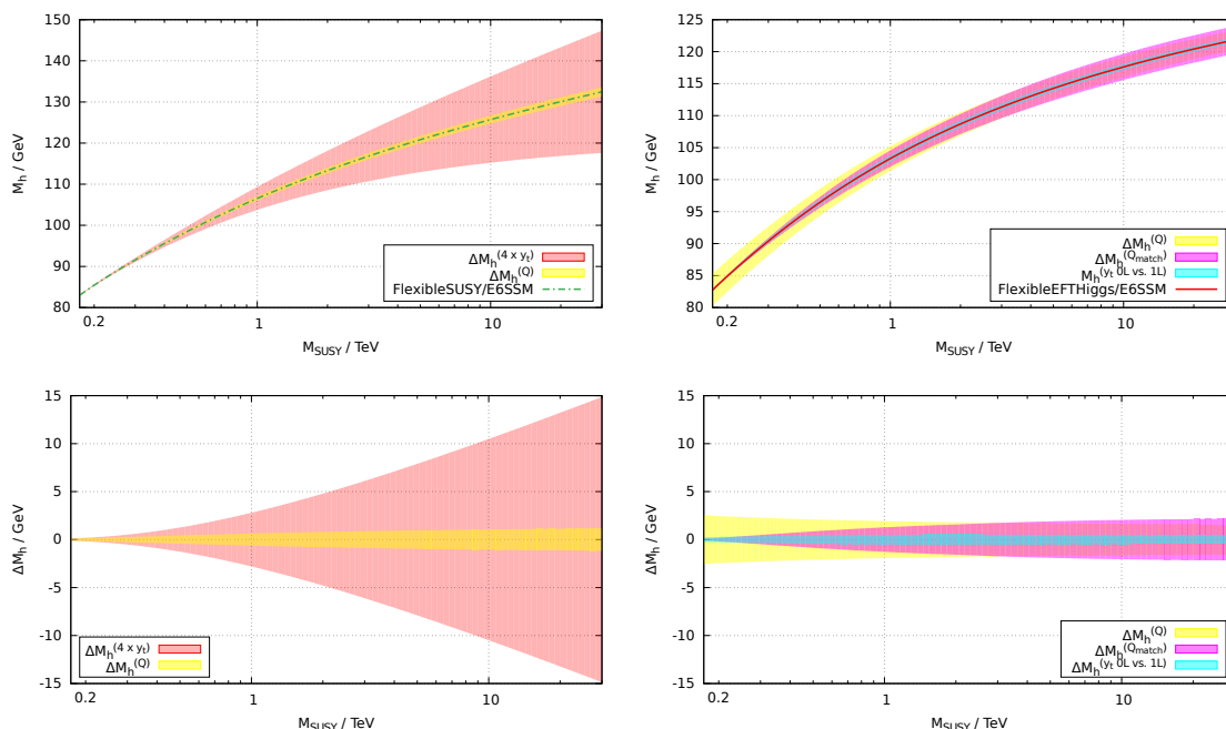
Figure 12. Higgs mass predictions and uncertainty estimates of section 3 applied to the fixed-order calculations with FlexibleSUSY and to FlexibleEFTHiggs in the E_6 SSM with fixed X_t = 0 , \tan \beta = 5 and \lambda = 0.1 . The top row shows the Higgs mass predictions and the uncertainty estimates, the lower row only the uncertainty estimates, as in figure 7.
