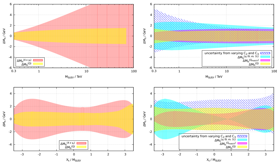
Figure 7. Uncertainty estimates for the fixed-order 2-loop calculations with FlexibleSUSY and SARAH/SPheno and for FlexibleEFTHiggs. Left panels: fixed-order uncertainty estimates of section 3.1.2 using renormalization scale variation, \Delta M_h^{(Q)} (yellow) and from the different top Yukawa definitions, \Delta M_h^{(4 \times y_t)} (red). Right panels: FlexibleEFTHiggs uncertainty estimations of section 3.2.2 using renormalization scale uncertainty, \Delta M_h^{(Q)} (yellow), matching scale variation, \Delta M_h^{(Q_{\text{match}})} (pink) and the uncertainty from different loop orders for the top pole mass matching, \Delta M_h^{(y_t \text{ 0L vs. 1L})} (turquoise). In the top row \tan \beta = 5 and X_t = -2M_{\text{SUSY}} is used. In the bottom row we set \tan \beta = 5 and M_{\text{SUSY}} = 2 \text{ TeV} .
