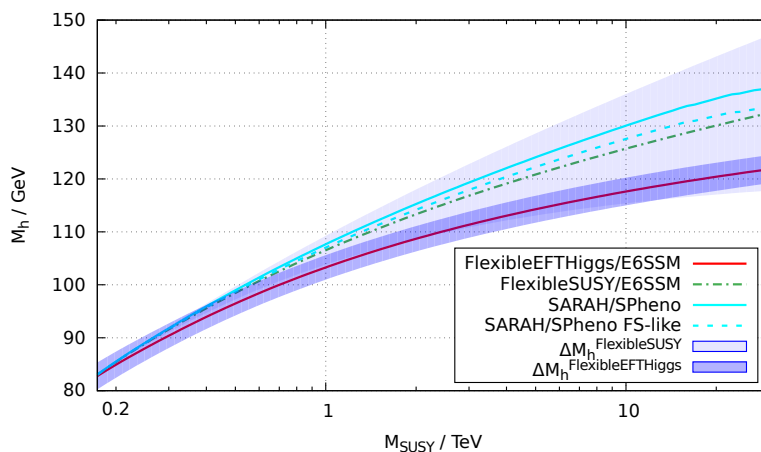
Figure 13. Predictions for M_h and combined theoretical uncertainty estimates for FlexibleSUSY and FlexibleEFTHiggs in the E_6 SSM, compared with results of other codes. We fix X_t = 0 , \tan \beta = 5 and \lambda = 0.1 .
