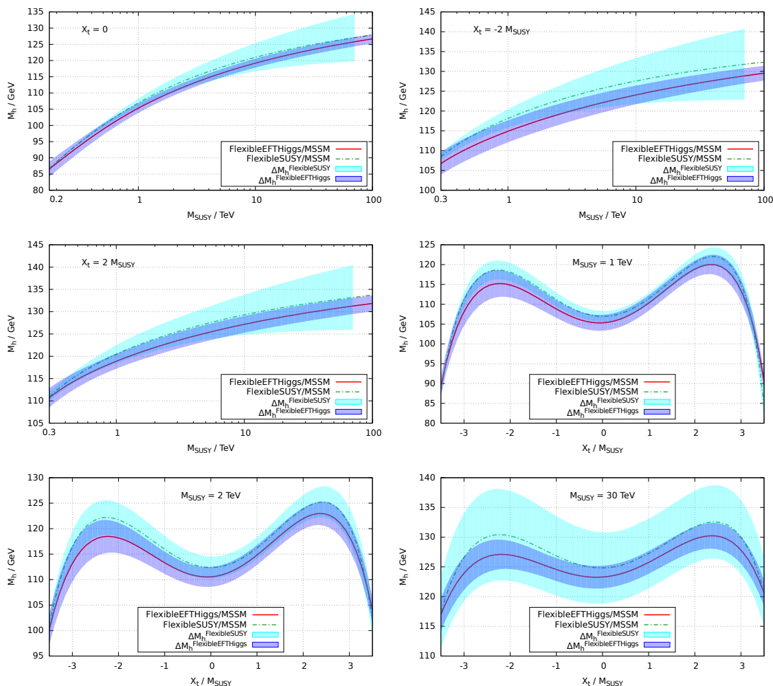
Figure 8. Predictions for M_h and combined theoretical uncertainty estimates for FlexibleSUSY and FlexibleEFTHiggs in the MSSM for \tan\beta = 5 . The first three panels show M_h as a function of M_{\text{SUSY}} for X_t/M_{\text{SUSY}} = 0, -2 and 2 , respectively. The last three panels show M_h as a function X_t for M_{\text{SUSY}} = 1 \text{ TeV}, 2 \text{ TeV} and 30 \text{ TeV} , respectively.
