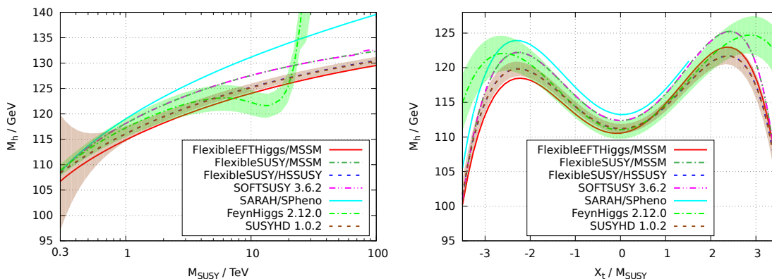
Figure 6. Comparison of predictions for M_h in the MSSM using the EFT with pole mass matching method (FlexibleEFTHiggs/MSSM), the pure EFT calculation (FlexibleSUSY/HSSUSY and SUSYHD) and the diagrammatic calculations (FlexibleSUSY/MSSM, SARAH/SPheno, SOFTSUSY and FeynHiggs) for \tan\beta = 5 . The green and brown bands show the theory uncertainty as estimated by FeynHiggs and SUSYHD, respectively. In the left panel we fix X_t = -2M_{\text{SUSY}} and vary M_{\text{SUSY}} . In the right panel we fix M_{\text{SUSY}} = 2\text{ TeV} and vary X_t .
