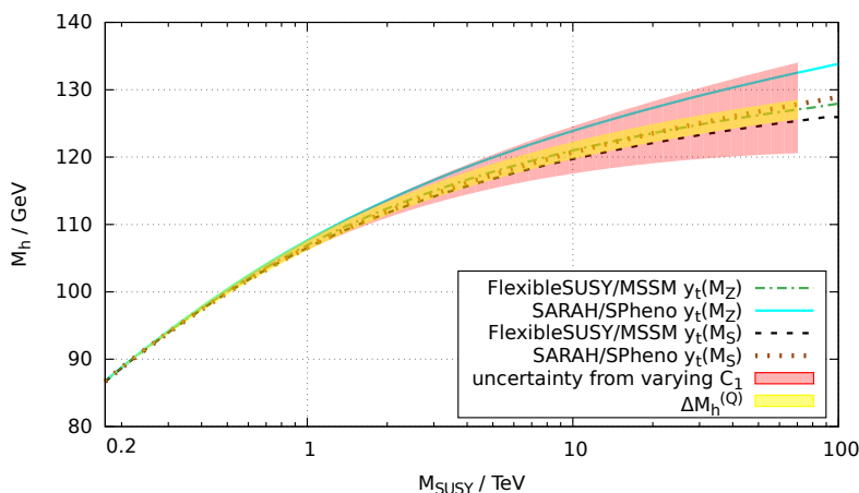
Figure 4. Illustration of the theory uncertainty estimate \Delta M_h^{(4 \times y_t)} of the fixed-order calculations of FlexibleSUSY and SARAHS/SPHeno using four different ways to calculate y_t^{\text{MSSM}} . We choose \tan\beta = 5 and X_t = 0 . The red band shows the variation of M_h when the coefficient C_1 is varied within the interval [-184/9, 184/9] . The yellow uncertainty band shows \Delta M_h^{(Q)} , defined as the variation of M_h when the renormalization scale at which M_h is calculated is varied within [M_{\text{SUSY}}/2, 2M_{\text{SUSY}}] .
