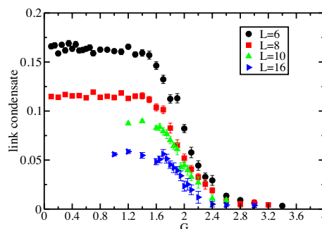
Figure 10. O_1 vs. G with temporal apbc.
