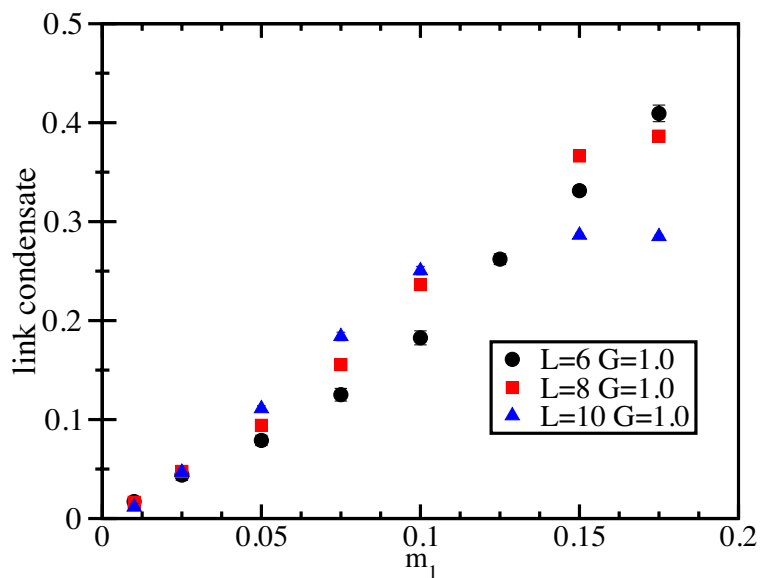
Figure 4. \langle O_1 \rangle vs m_1 at G = 1.0 for L = 6, 8, 10 and pbc.
