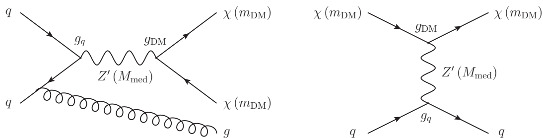
Figure 1. The left diagram shows a contributing diagram for mono-jet production with an (axial) vector mediator at a hadron collider. The process is characterised by M_{\text{med}} , m_{\text{DM}} , g_{\text{DM}} and g_q , which are the mediator and dark matter masses, and the mediator couplings to dark matter and quarks respectively. The right diagram shows the corresponding scattering process relevant for direct detection, which is characterised by the same four parameters.
