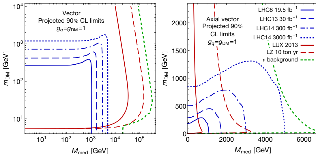
Figure 10. The blue and red lines show the current and projected 90% CL limits from the LHC mono-jet and LUX searches in the m_{DM} vs M_{med} plane. The left and right panels show the limits for vector and axial-vector mediators respectively for (g_q, g_{DM}) = (1, 1) . The region to the left of the various curves is excluded. The plot legend is the same for both panels. The short-dashed green lines shows the direct detection discovery reach after accounting for the neutrino background. While LUX has better sensitivity than mono-jet searches and approaches the neutrino limit for vector mediators, the opposite is true for axial-vector mediators. Note that the left (right) panel has log (linear) axes.
