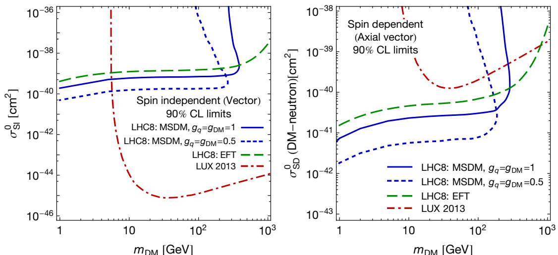
Figure 12. A comparison between the 90% CL mono-jet limit in our MSDM models (blue lines) and the EFT framework (green dashed) in the cross-section vs m_{\text{DM}} plane used by the direct detection community. The left and right panels show the limits on the SI and SD cross-sections appropriate for vector and axial-vector mediators respectively. The red dot-dashed line shows the current LUX limit. The MSDM and EFT limits should agree in the domain where the EFT framework is valid. For these choices of parameters, the EFT limit underestimates the MSDM limits for m_{\text{DM}} \lesssim 300 GeV and overestimates them for m_{\text{DM}} \gtrsim 300 GeV. The EFT limit gives a misleading representation of the relative sensitivity of mono-jet and direct detection searches.
