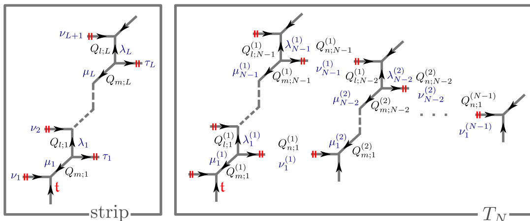
Figure 23. The left part of the figure shows the strip diagram, while the right one depicts the dissection of the T_N diagram into N strips. The partitions associated with the horizontal, diagonal and vertical lines are \nu_i^{(j)} , \mu_i^{(j)} and \lambda_i^{(j)} with j = 1, \dots, N - 1 , i = 1, \dots, N - j respectively. The Kähler parameters of the horizontal, diagonal and vertical lines are Q_{n;i}^{(j)} , Q_{m;i}^{(j)} , Q_{l;i}^{(j)} respectively with the same range of indices.
