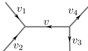
Figure 10. This figure gives an example for the determination v_{in} and v_{out} .
