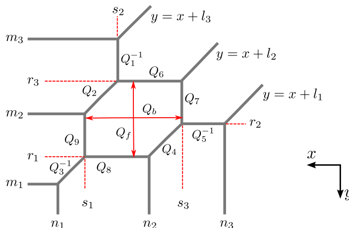
Figure 26. This figure illustrates the parametrization of the Kähler moduli as functions of the toric geometry. The equations y = x + l_i come from the conditions \tilde{W} = -\tilde{L}_i \tilde{T} .
