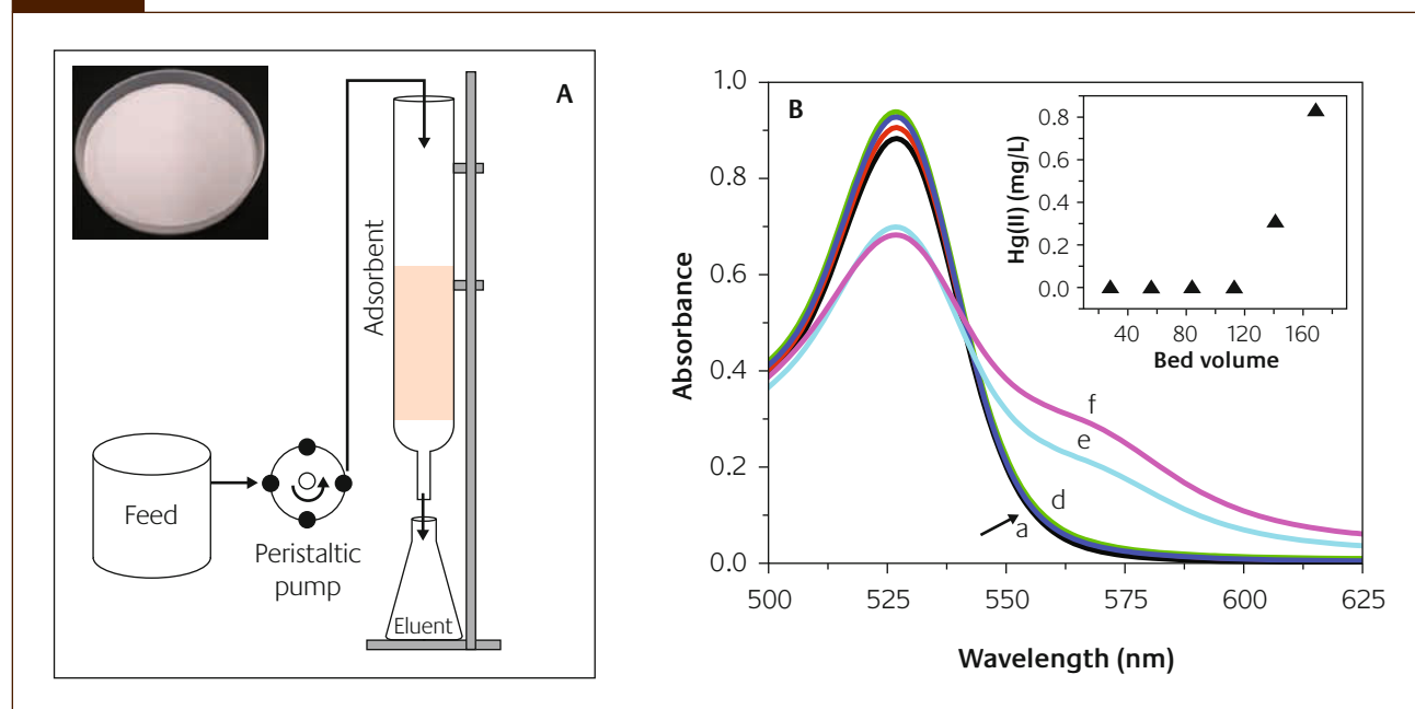
(A) Schematic representation of the down-flow column apparatus. Inset is a photograph of gold nanoparticle-supported alumina. (B) UV-vis absorption spectra of the solution as 1.0 mg/L Hg(II) was flown through the column. Traces 'a-d' are the absorption spectra corresponding to the passage of 0.10, 0.20, 0.30 and 0.40 L, respectively. Trace 'e' is for 0.5 L and trace 'f' is for 0.6 L, respectively. Inset is the plot of concentration versus bed volume
