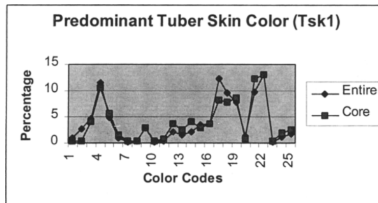
FIGURE 1. Frequency distribution (%) of predominant tuber skin colors in whole and core collection of S. tuberosum subsp. andigena . Table 3 lists the color codes for this characteristic.
