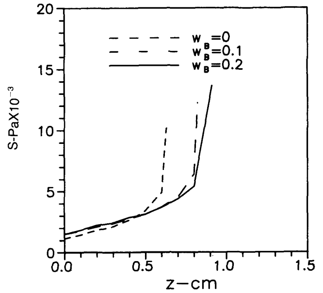
Fig. 13—Surface tension pressure distributions for different weight percents of volatile alloying element ( Q = 3 kW, U = 2 cm/s, \beta = 0 , and f = 0 ).
