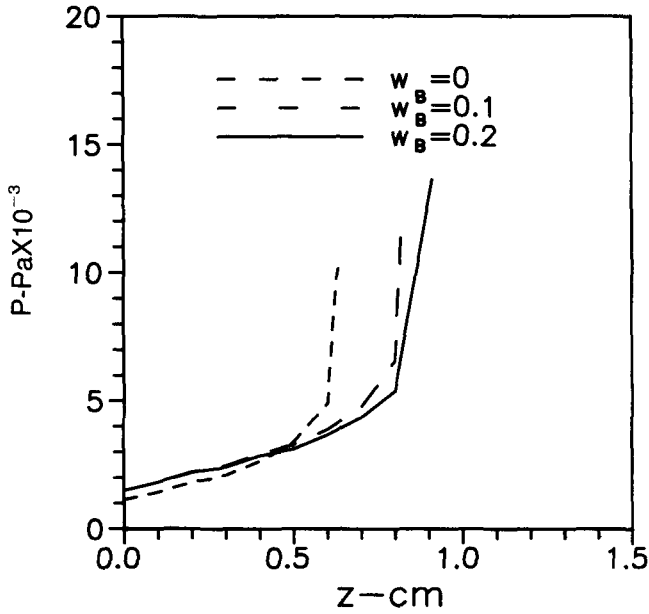
Fig. 12—Total vapor pressure distributions for different weight percents of volatile alloying element ( Q = 3 kW, U = 2 cm/s, \beta = 0 , and f = 0 ).
