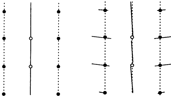
Fig. 3. Removing degeneracies.
