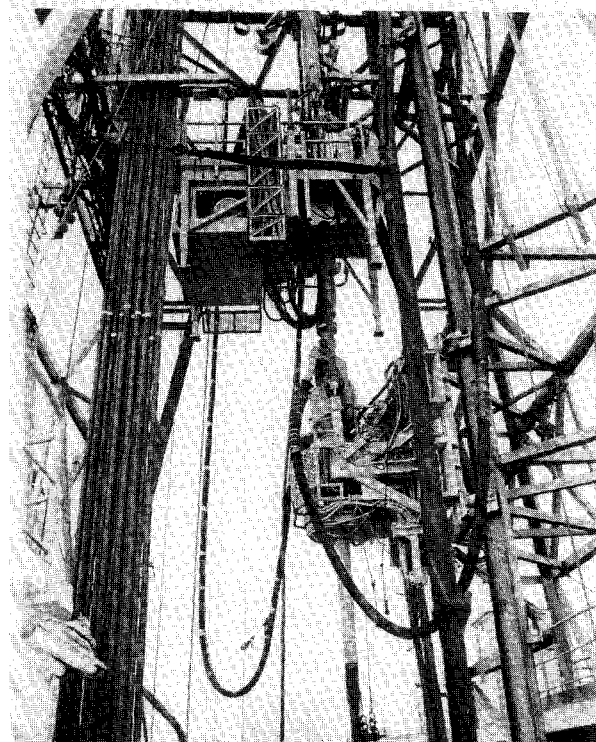
Fig. 25. Diamond Coring System (DCS) top drive concept.
