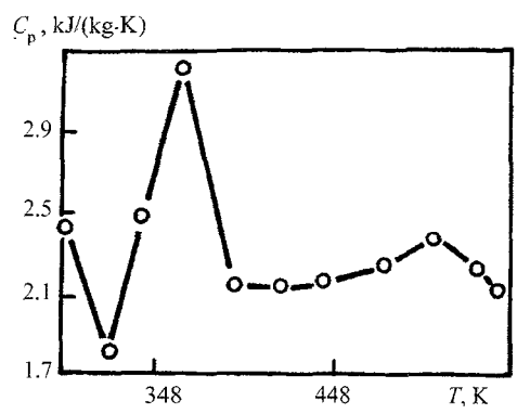
Fig. 1. Specific heat capacity ( C_p ) of stuffing box packing impregnated with ceresine vs. temperature.
