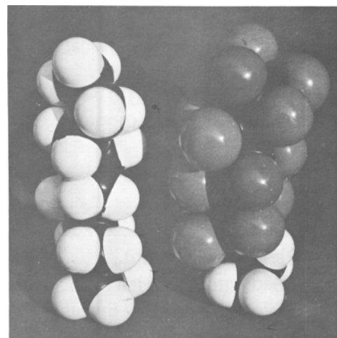
Fig. 7 Comparison of straight alkyl chain with fluorinated ligand which is unable to cluster.
