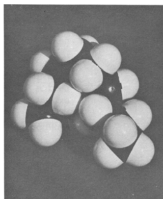
Fig. 6 Crowded n-C 10 H 21 -chain producing rather plain area.
