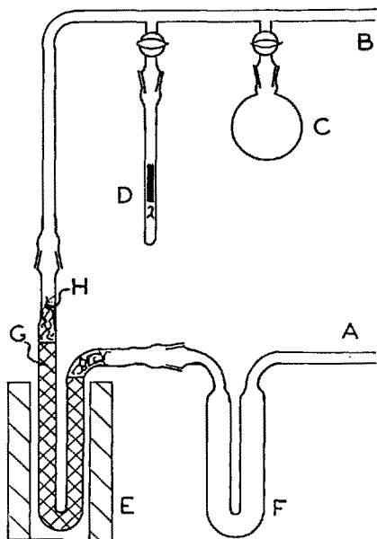
Apparatus for the preparation of tritiated water. A , intake of Toeppler pump; B , outlet of Toeppler pump; C , flask containing 1-3 ml of ordinary water; D , ampoule holding tritium, and a magnet; E , furnace; F , cold-trap; G , copper-oxide wire; H , glass wool.
