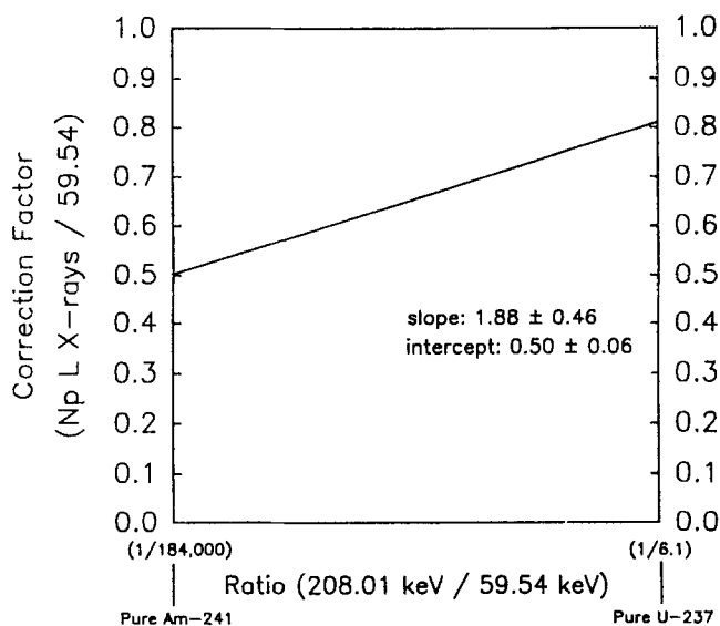
Fig. 4. Linear relationship for the determination of the Np L X-ray correction factor
