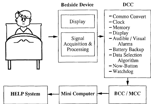
Fig. 2. MIB Block Diagram, where: DCC = Device Communications Controller, BCC = Bedside Communications Controller, MCC = Master Communications Controller.
