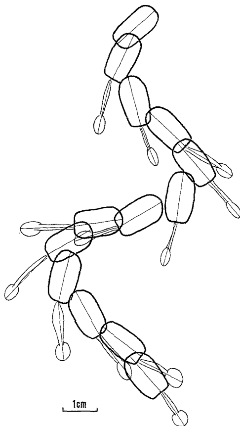
Fig. 3: Lateral view of Euphysa flammea during turning, after milk has been injected into the subumbrellar cavity to show the direction of expulsion of subumbrellar water during the early part of the contraction. Each outline shows the subumbrella shortly after the beginning of a contraction. The jet of milky water in each case is directed at an angle to the axis of the bell such that a net force is exerted on the wall on the outside of the turn. Traced from cine sequences
