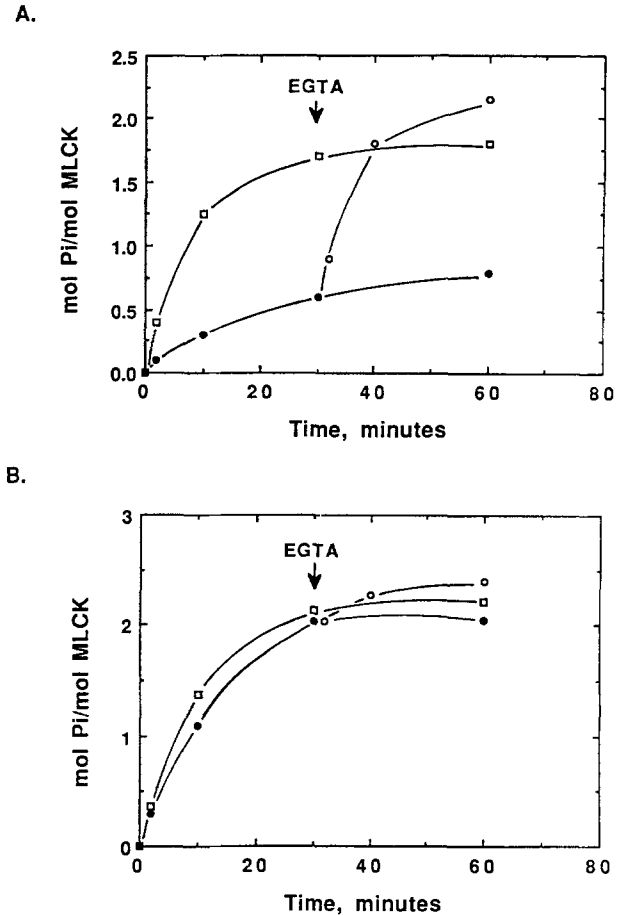
Fig. 1. Time course of phosphorylation of MLCK from turkey gizzards (A) and pregnant sheep myometrium (B) by PKA in the absence (□) and presence (●) of bound \text{Ca}^{2+} -calmodulin as described in the 'Materials and methods'. After 30 min of phosphorylation, half of the latter reaction mixture containing \text{Ca}^{2+} -calmodulin was made to 1 mM EGTA (○). Aliquots of the reaction mixtures were taken at the times indicated for determination of phosphate incorporation.
