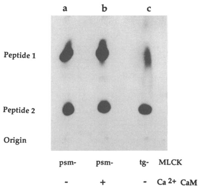
Fig. 2. Autoradiograph of ^{32}\text{P} -labeled tryptic peptides of psmMLCK after thin layer cellulose electrophoresis. Aliquots of the reaction mixtures in Fig. 1 were taken after 60 min incubation, lyophilized and digested with trypsin as described in the 'Materials and methods'. The tryptic peptides of psmMLCK (lanes a and b) and tgMLCK (lane c) phosphorylated by PKA in the absence (lanes a and c) and presence (lane b) of \text{Ca}^{2+} -calmodulin were subjected to thin layer electrophoresis.
