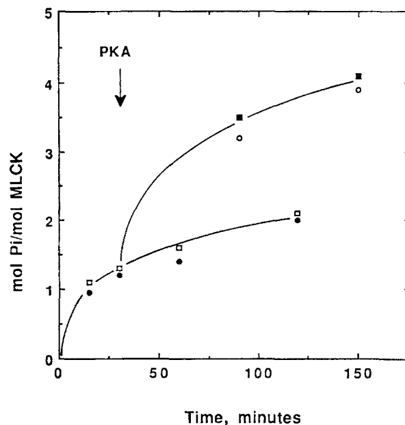
Fig. 3. Time course of phosphorylation of psmMLCK by PKC and PKA. Phosphorylation of psmMLCK by PKC was carried out in the presence (□) and absence (●) of \text{Ca}^{2+} -calmodulin. After 30 min of incubation, PKA was added to half of the reaction mixtures (■, ○). Aliquots were taken for determination of phosphate incorporation.
