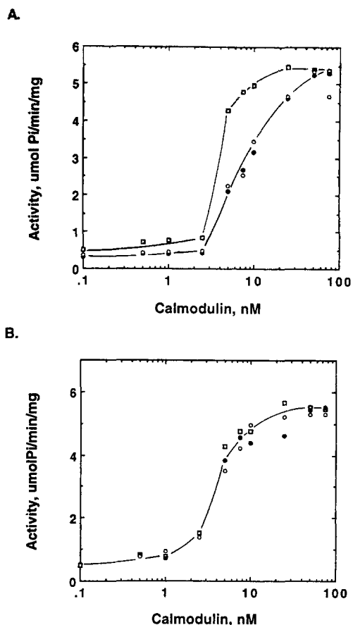
Fig. 5. Activation by calmodulin of unphosphorylated psmMLCK ( \square ), psmMLCK phosphorylated in the presence ( \bullet ) and absence ( \circ ) of \text{Ca}^{2+} -calmodulin by PKA (A) and PKC (B). Following incubation of psmMLCK with PKA for 60 min as described in Fig. 1B and with PKC for 2 h as described in Fig. 3, the MLCK activity was determined at various calmodulin concentration.
