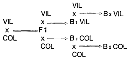
Fig. 2. Outline of the experimental crossing program carried out in Armeria . COL A. colorata , VIL A. villosa subsp. longiaristata
