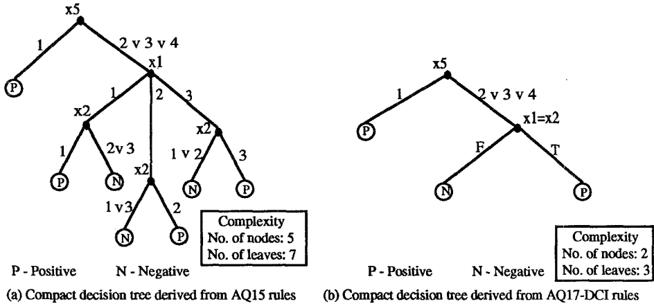
Figure 9. Compact decision trees generated by AQDT-1 for the MONK-1 problem
