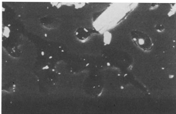
Figure 3 Back-scattered electron micrograph of a ZrO_2 -modified epoxy polymer which had been polished to reveal the profile of crack surfaces ( \times 475 ).
