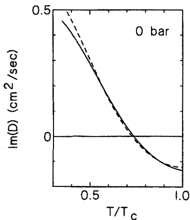
Fig. 12. Imaginary part of the spin diffusion coefficient of the B phase at 0 bar and a Larmor frequency of 2 MHz. (—) Experimental results obtained by fitting to the spin-wave peak frequencies as in Fig. 11. (--) The theoretical predictions of ref. 7, recalculated with values of F_0^3 and v_F from ref. 28.
