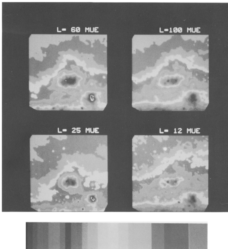
Fig. 2. IRAS maps of 5^\circ \times 5^\circ field centered on (l, b) = (18.5^\circ, 2.5^\circ) , near the HII region S54, at \lambda \mu\text{m} = 60, 100, 12, and 25 . The original colour wedge runs from purple through blue, green and yellow to red, either logarithmically (Figures 2, 3, 6, 7) or linearly (Figures 4, 5, 8); its gray-scale reproduction is shown underneath, increasing in intensity from left to right.
