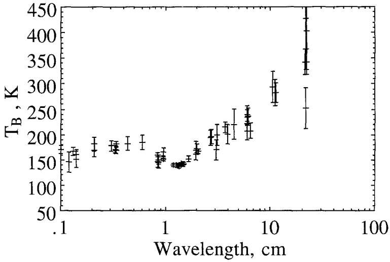
Figure 1. Jupiter's radio brightness temperature spectrum
