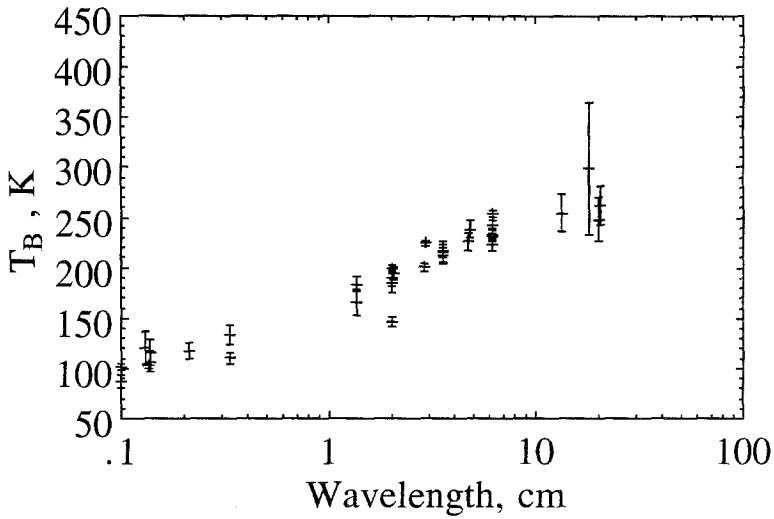
Figure 3. Uranus' radio brightness temperature spectrum
