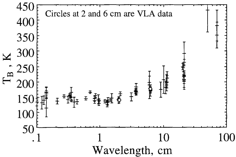
Figure 2. Saturn's radio brightness temperature spectrum
