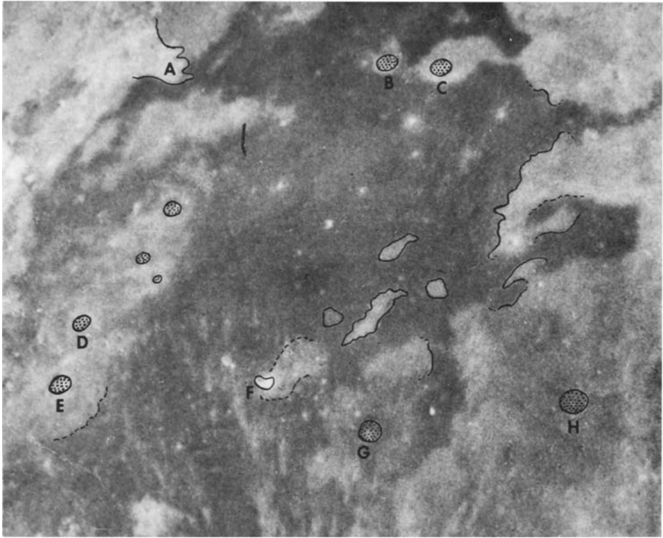
Fig. 4. Central and western Mare Imbrium, showing correspondence between color boundaries and flow fronts. A, Prom. Heraclides; B, Helicon; C, LeVerrier; D, Delisle; E, Diophantus; F, Mt. La Hire; G, Lambert; H, Timocharis.
