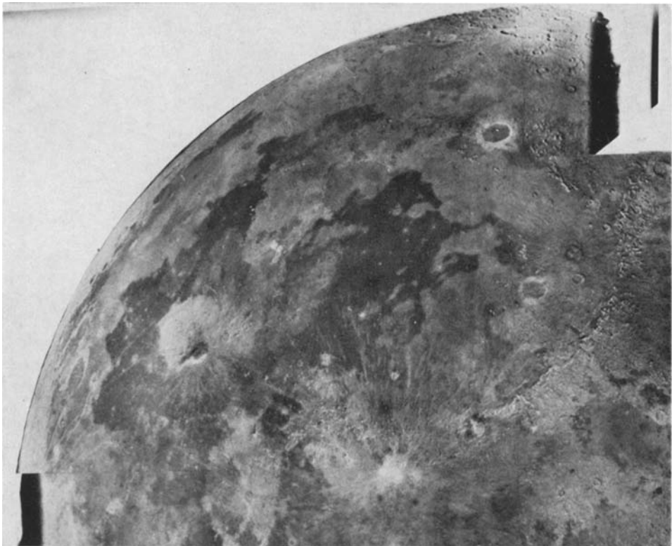
Fig. 1. IR minus UV composite photograph of Moon's NW quadrant. Redder regions, such as the walls of Plato and Wood's Spot near Aristarchus, appear lighter.
