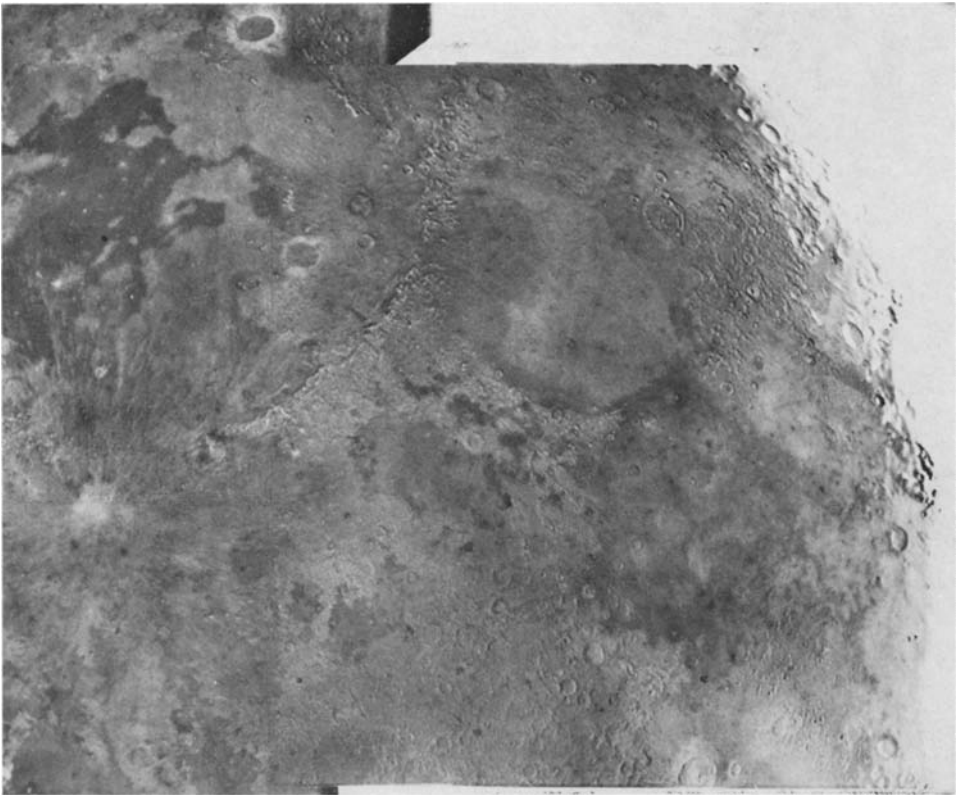
Fig. 3. Composite photograph of NE portion of Moon. The low sun angle gives spurious effects in shadows and bright crater rims.
