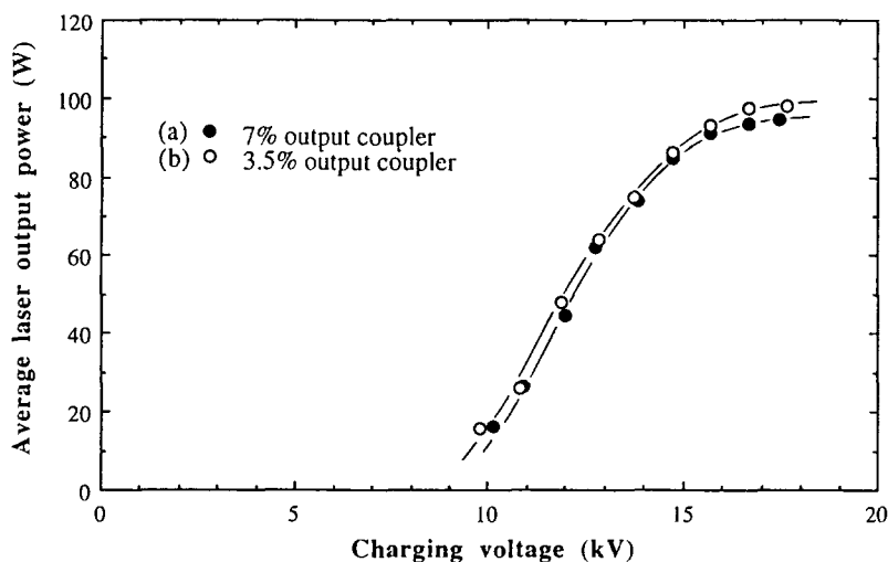
Figure 5 The dependence of laser output power on charging voltage for configuration (a), a 7% reflecting output coupler, and configuration (b), a 3.5% reflecting output coupler. The window reflection losses at each end were about 7% (neglecting interference effects). Laser operating parameters were as described for Fig. 3.
